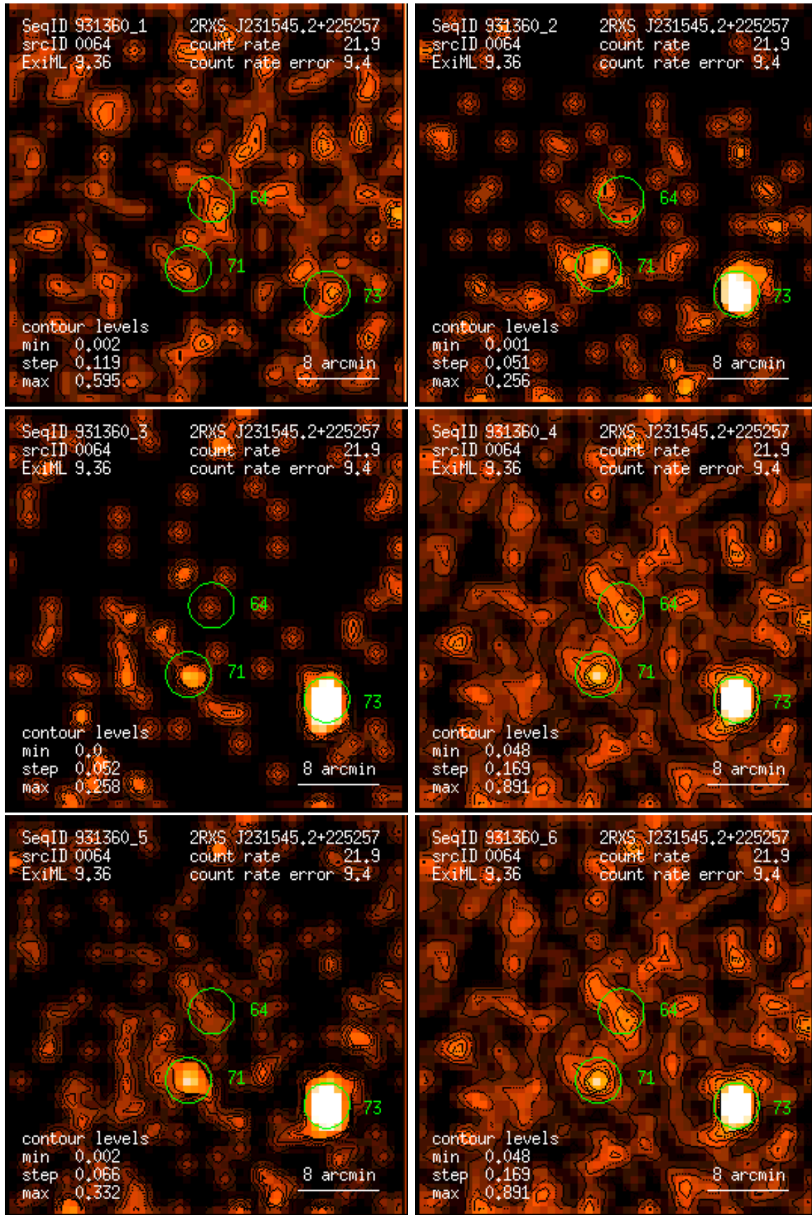
Figure 64: RASS 931360: detection 0064: band rate images, Gaussian filter: (1) PSPC channels 11 – 41, (2) 52 – 90, (3) 91 – 201, (4) 11 – 235, (5) 52 – 201, (6) 11 – 201. Broad band rates in counts/ks. Band rate contour levels in counts/ks/arcmin 2 .
