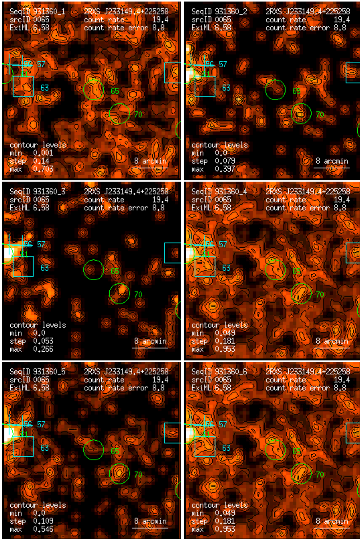
Figure 65: RASS 931360: detection 0065: band rate images, Gaussian filter: (1) PSPC channels 11 – 41, (2) 52 – 90, (3) 91 – 201, (4) 11 – 235, (5) 52 – 201, (6) 11 – 201. Broad band rates in counts/ks. Band rate contour levels in counts/ks/arcmin 2 .
