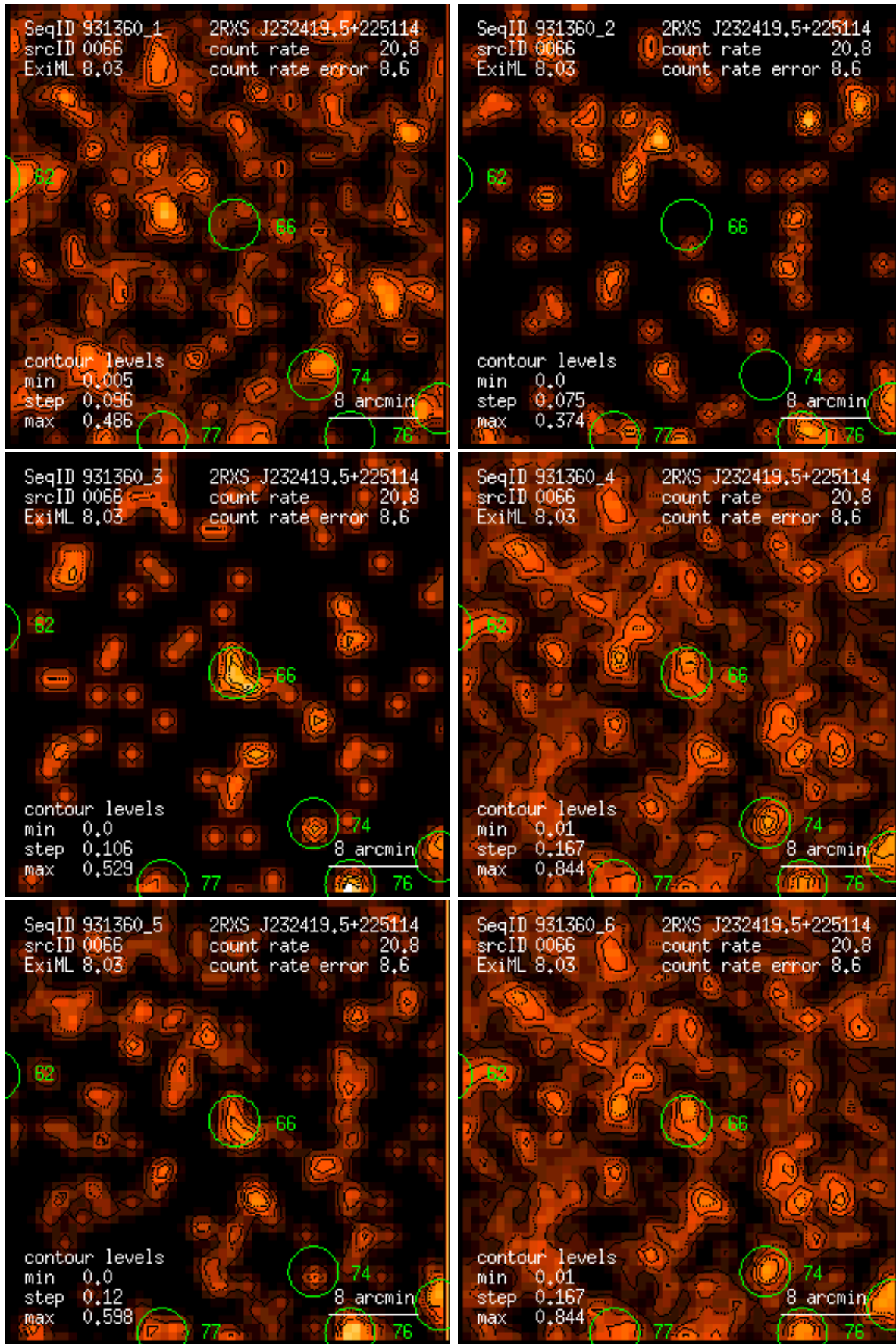
Figure 66: RASS 931360: detection 0066: band rate images, Gaussian filter: (1) PSPC channels 11 – 41, (2) 52 – 90, (3) 91 – 201, (4) 11 – 235, (5) 52 – 201, (6) 11 – 201. Broad band rates in counts/ks. Band rate contour levels in counts/ks/arcmin 2 .
