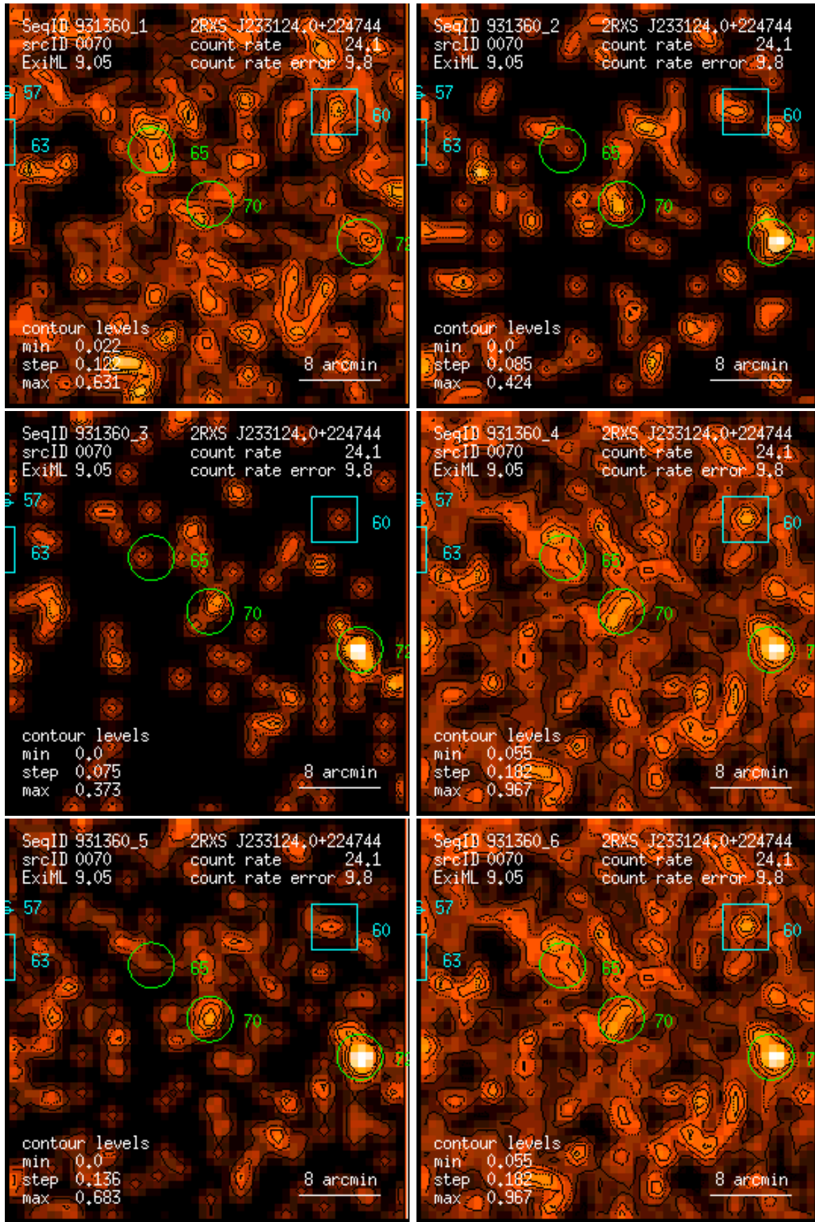
Figure 70: RASS 931360: detection 0070: band rate images, Gaussian filter: (1) PSPC channels 11 – 41, (2) 52 – 90, (3) 91 – 201, (4) 11 – 235, (5) 52 – 201, (6) 11 – 201. Broad band rates in counts/ks. Band rate contour levels in counts/ks/arcmin 2 .
