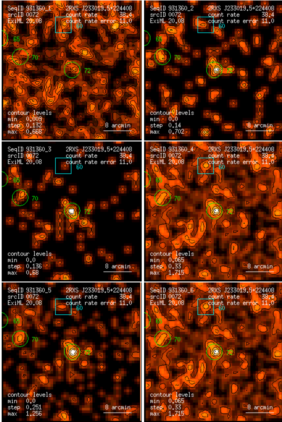
Figure 72: RASS 931360: detection 0072: band rate images, Gaussian filter: (1) PSPC channels 11 – 41, (2) 52 – 90, (3) 91 – 201, (4) 11 – 235, (5) 52 – 201, (6) 11 – 201. Broad band rates in counts/ks. Band rate contour levels in counts/ks/arcmin 2 .
