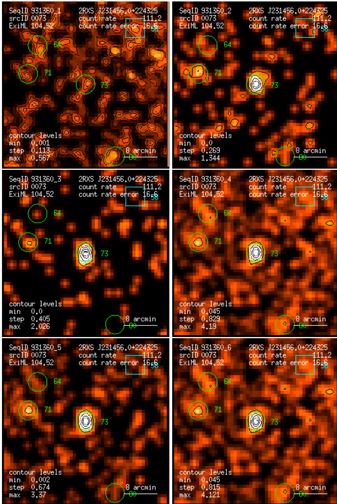
Figure 73: RASS 931360: detection 0073: band rate images, Gaussian filter: (1) PSPC channels 11 – 41, (2) 52 – 90, (3) 91 – 201, (4) 11 – 235, (5) 52 – 201, (6) 11 – 201. Broad band rates in counts/ks. Band rate contour levels in counts/ks/arcmin 2 .
