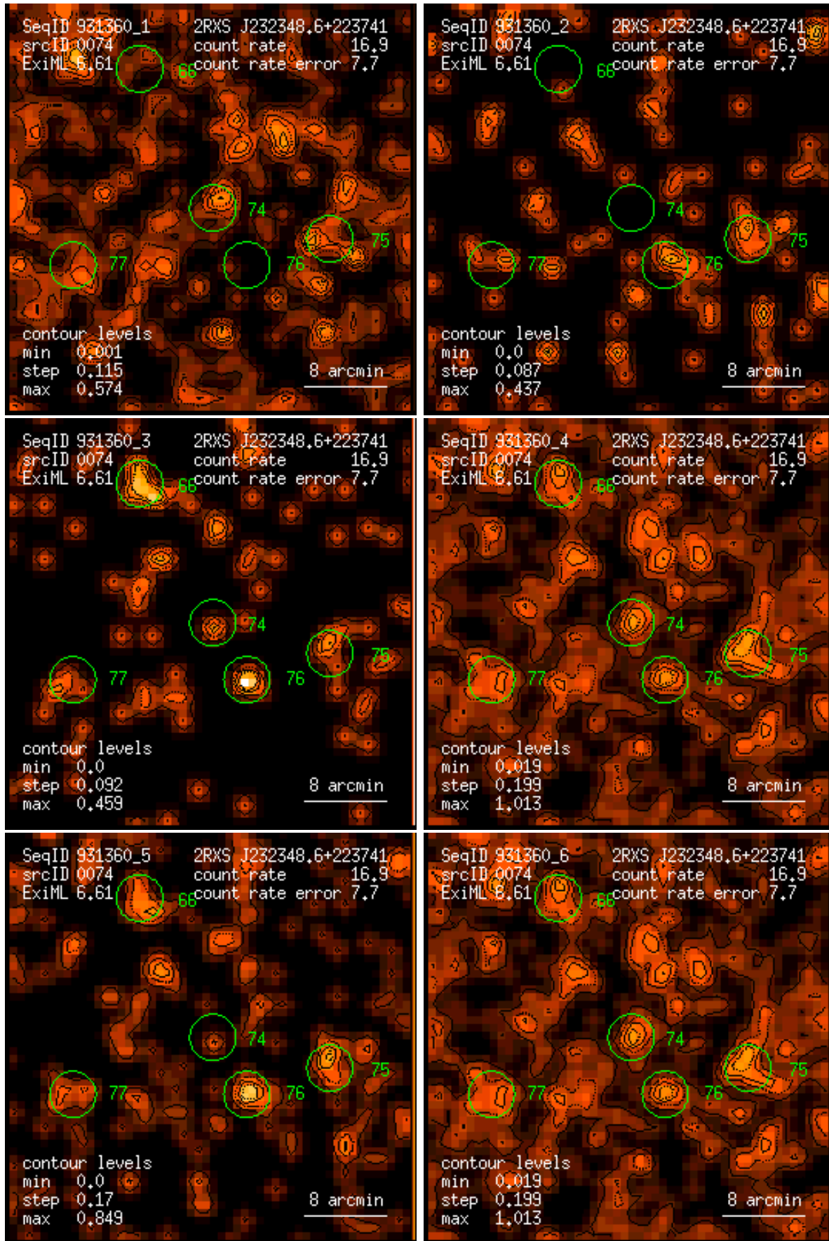
Figure 74: RASS 931360: detection 0074: band rate images, Gaussian filter: (1) PSPC channels 11 – 41, (2) 52 – 90, (3) 91 – 201, (4) 11 – 235, (5) 52 – 201, (6) 11 – 201. Broad band rates in counts/ks. Band rate contour levels in counts/ks/arcmin 2 .
