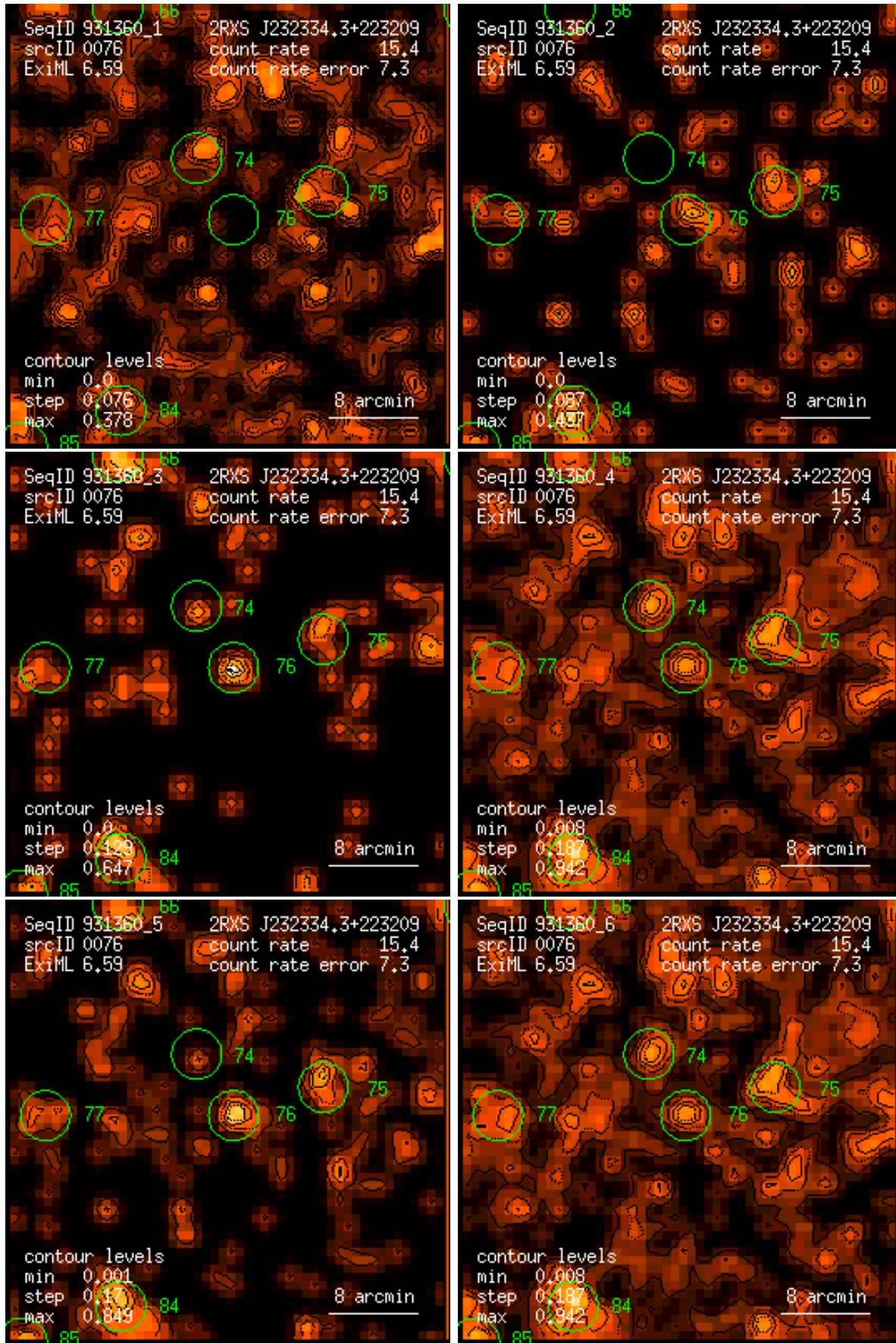
Figure 76: RASS 931360: detection 0076: band rate images, Gaussian filter: (1) PSPC channels 11 – 41, (2) 52 – 90, (3) 91 – 201, (4) 11 – 235, (5) 52 – 201, (6) 11 – 201. Broad band rates in counts/ks. Band rate contour levels in counts/ks/arcmin 2 .
