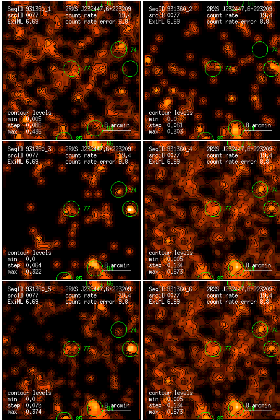
Figure 77: RASS 931360: detection 0077: band rate images, Gaussian filter: (1) PSPC channels 11 – 41, (2) 52 – 90, (3) 91 – 201, (4) 11 – 235, (5) 52 – 201, (6) 11 – 201. Broad band rates in counts/ks. Band rate contour levels in counts/ks/arcmin 2 .
