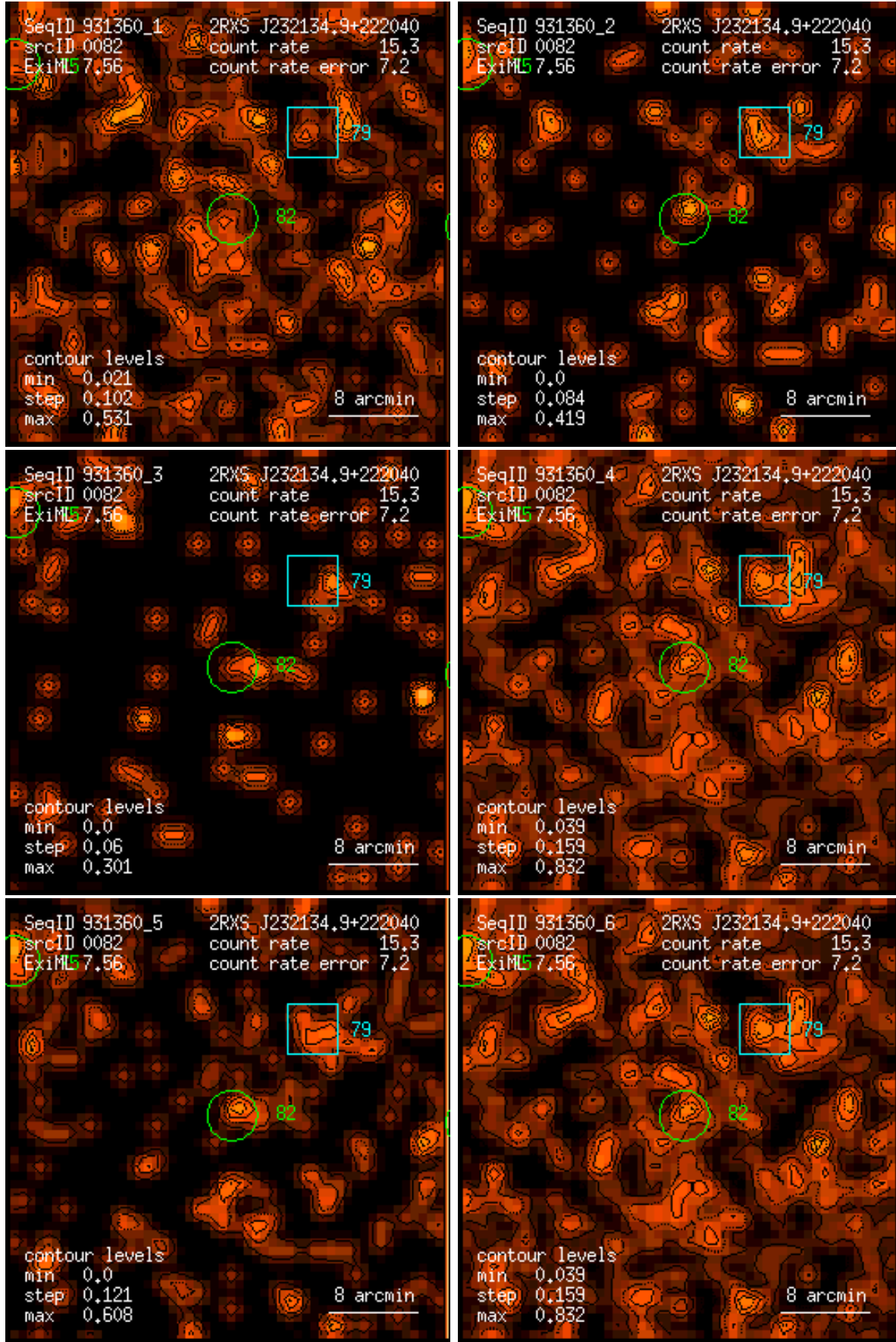
Figure 82: RASS 931360: detection 0082: band rate images, Gaussian filter: (1) PSPC channels 11 – 41, (2) 52 – 90, (3) 91 – 201, (4) 11 – 235, (5) 52 – 201, (6) 11 – 201. Broad band rates in counts/ks. Band rate contour levels in counts/ks/arcmin 2 .
