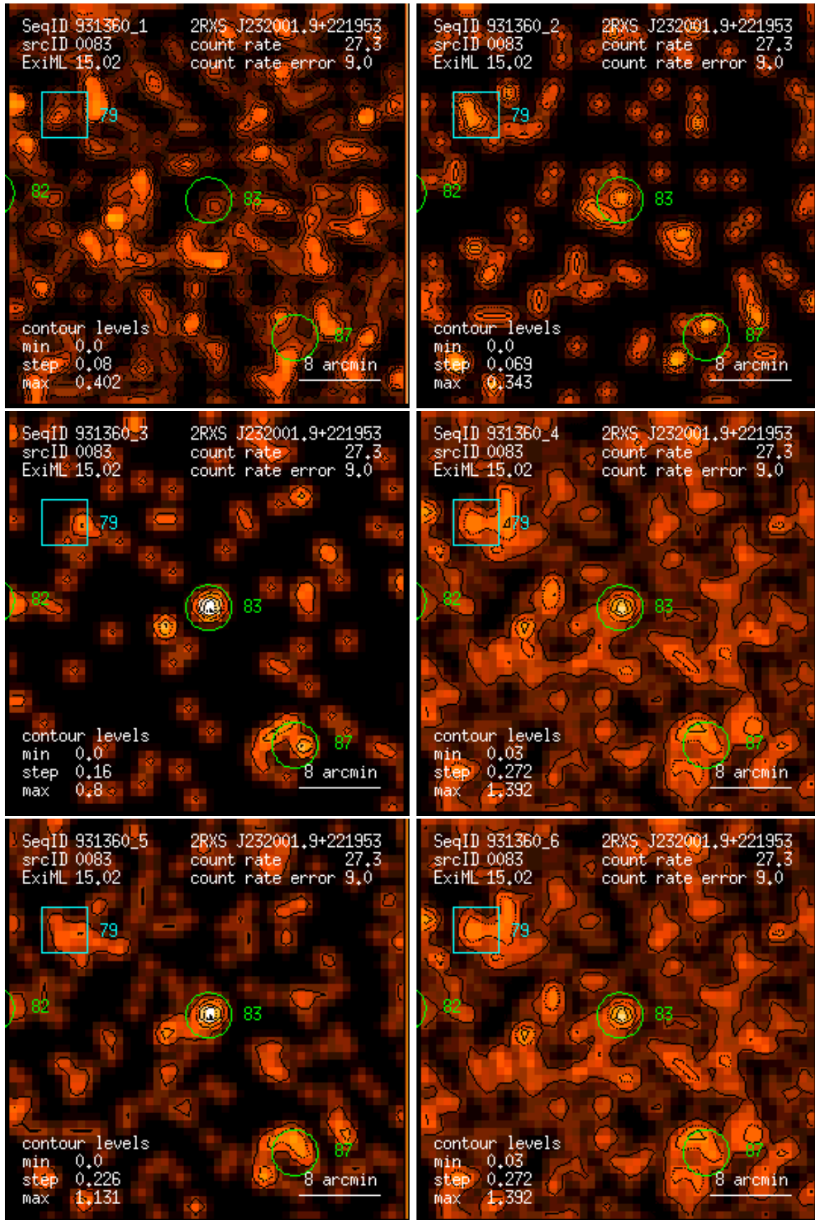
Figure 83: RASS 931360: detection 0083: band rate images, Gaussian filter: (1) PSPC channels 11 – 41, (2) 52 – 90, (3) 91 – 201, (4) 11 – 235, (5) 52 – 201, (6) 11 – 201. Broad band rates in counts/ks. Band rate contour levels in counts/ks/arcmin 2 .
