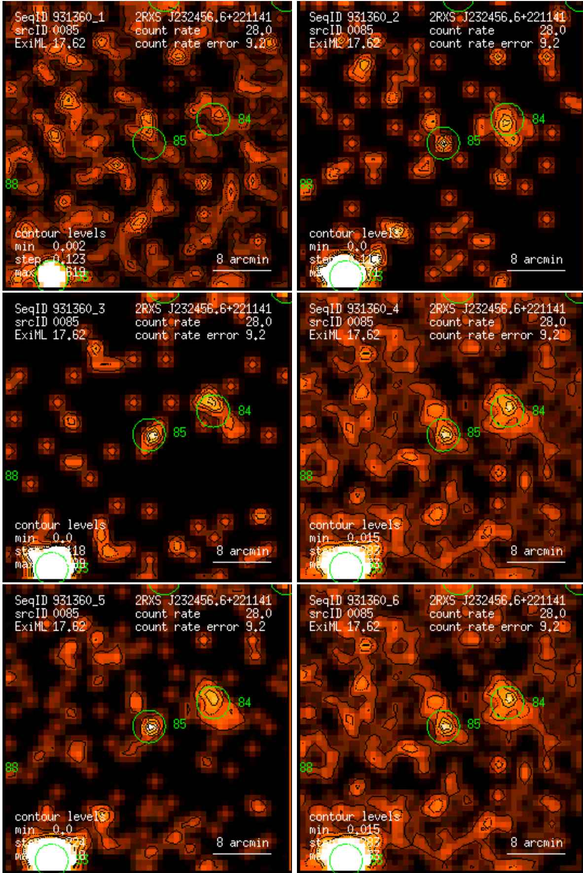
Figure 85: RASS 931360: detection 0085: band rate images, Gaussian filter: (1) PSPC channels 11 – 41, (2) 52 – 90, (3) 91 – 201, (4) 11 – 235, (5) 52 – 201, (6) 11 – 201. Broad band rates in counts/ks. Band rate contour levels in counts/ks/arcmin 2 .
