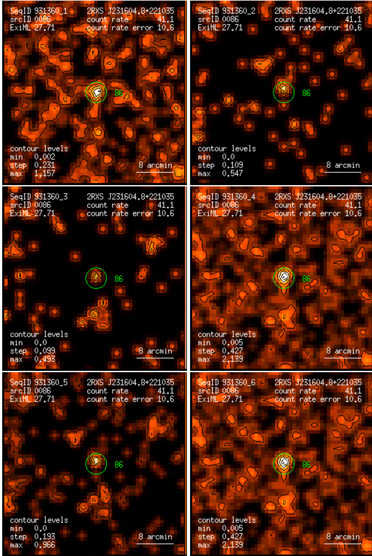
Figure 86: RASS 931360: detection 0086: band rate images, Gaussian filter: (1) PSPC channels 11 – 41, (2) 52 – 90, (3) 91 – 201, (4) 11 – 235, (5) 52 – 201, (6) 11 – 201. Broad band rates in counts/ks. Band rate contour levels in counts/ks/arcmin 2 .
