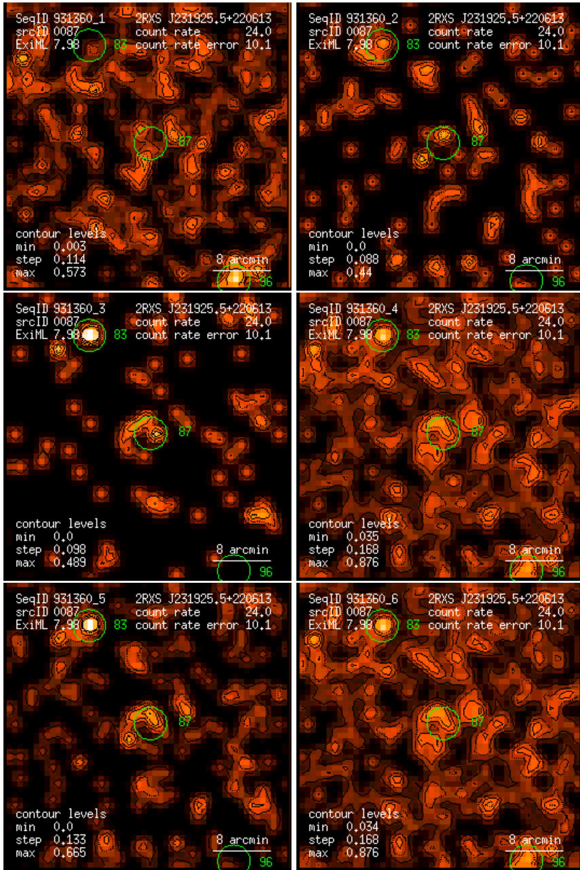
Figure 87: RASS 931360: detection 0087: band rate images, Gaussian filter: (1) PSPC channels 11 – 41, (2) 52 – 90, (3) 91 – 201, (4) 11 – 235, (5) 52 – 201, (6) 11 – 201. Broad band rates in counts/ks. Band rate contour levels in counts/ks/arcmin 2 .
