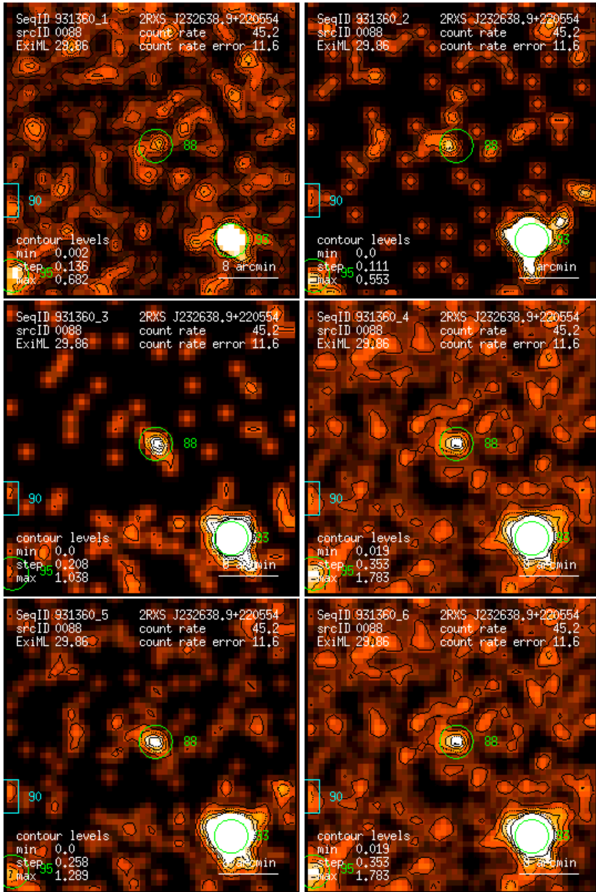
Figure 88: RASS 931360: detection 0088: band rate images, Gaussian filter: (1) PSPC channels 11 – 41, (2) 52 – 90, (3) 91 – 201, (4) 11 – 235, (5) 52 – 201, (6) 11 – 201. Broad band rates in counts/ks. Band rate contour levels in counts/ks/arcmin 2 .
