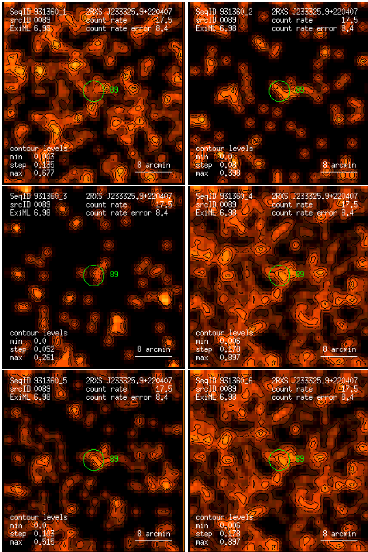
Figure 89: RASS 931360: detection 0089: band rate images, Gaussian filter: (1) PSPC channels 11 – 41, (2) 52 – 90, (3) 91 – 201, (4) 11 – 235, (5) 52 – 201, (6) 11 – 201. Broad band rates in counts/ks. Band rate contour levels in counts/ks/arcmin 2 .
