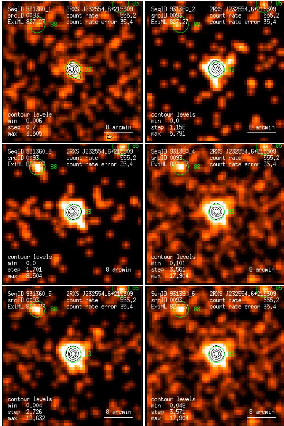
Figure 93: RASS 931360: detection 0093: band rate images, Gaussian filter: (1) PSPC channels 11 – 41, (2) 52 – 90, (3) 91 – 201, (4) 11 – 235, (5) 52 – 201, (6) 11 – 201. Broad band rates in counts/ks. Band rate contour levels in counts/ks/arcmin 2 .
