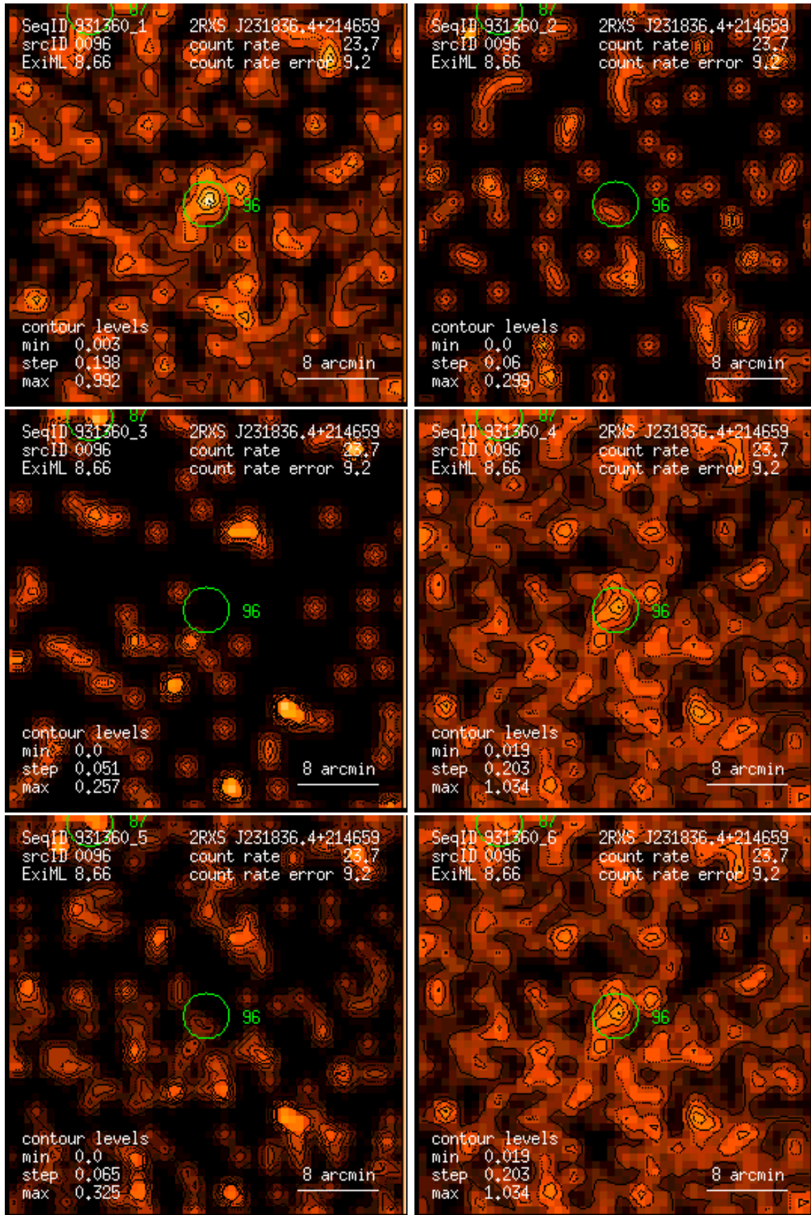
Figure 96: RASS 931360: detection 0096: band rate images, Gaussian filter: (1) PSPC channels 11 – 41, (2) 52 – 90, (3) 91 – 201, (4) 11 – 235, (5) 52 – 201, (6) 11 – 201. Broad band rates in counts/ks. Band rate contour levels in counts/ks/arcmin 2 .
