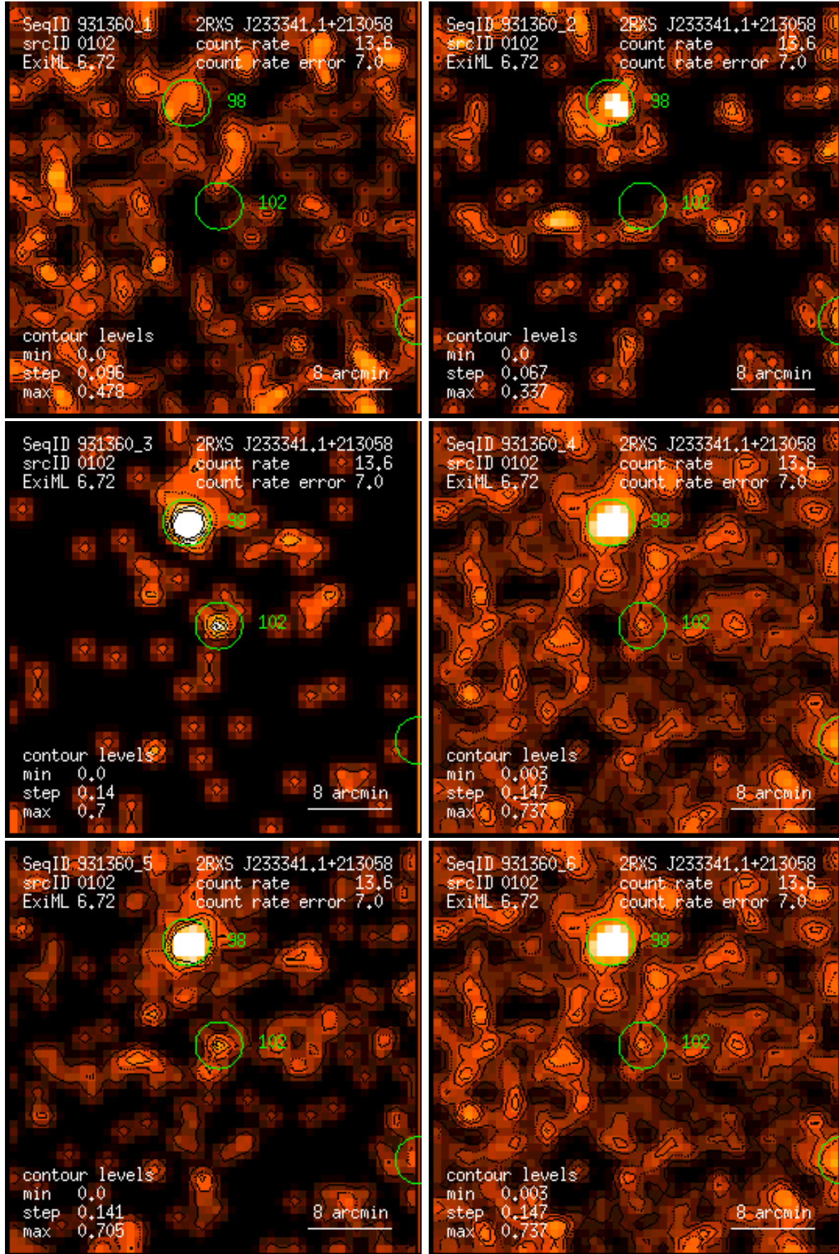
Figure 102: RASS 931360: detection 0102: band rate images, Gaussian filter: (1) PSPC channels 11 – 41, (2) 52 – 90, (3) 91 – 201, (4) 11 – 235, (5) 52 – 201, (6) 11 – 201. Broad band rates in counts/ks. Band rate contour levels in counts/ks/arcmin 2 .
