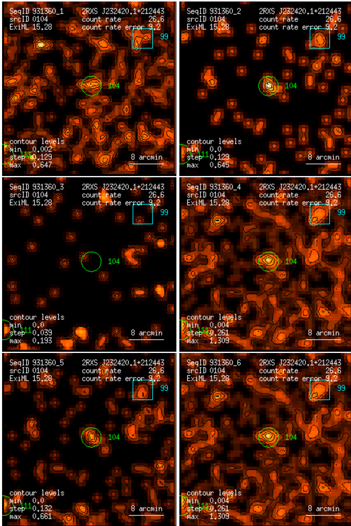
Figure 104: RASS 931360: detection 0104: band rate images, Gaussian filter: (1) PSPC channels 11 – 41, (2) 52 – 90, (3) 91 – 201, (4) 11 – 235, (5) 52 – 201, (6) 11 – 201. Broad band rates in counts/ks. Band rate contour levels in counts/ks/arcmin 2 .
