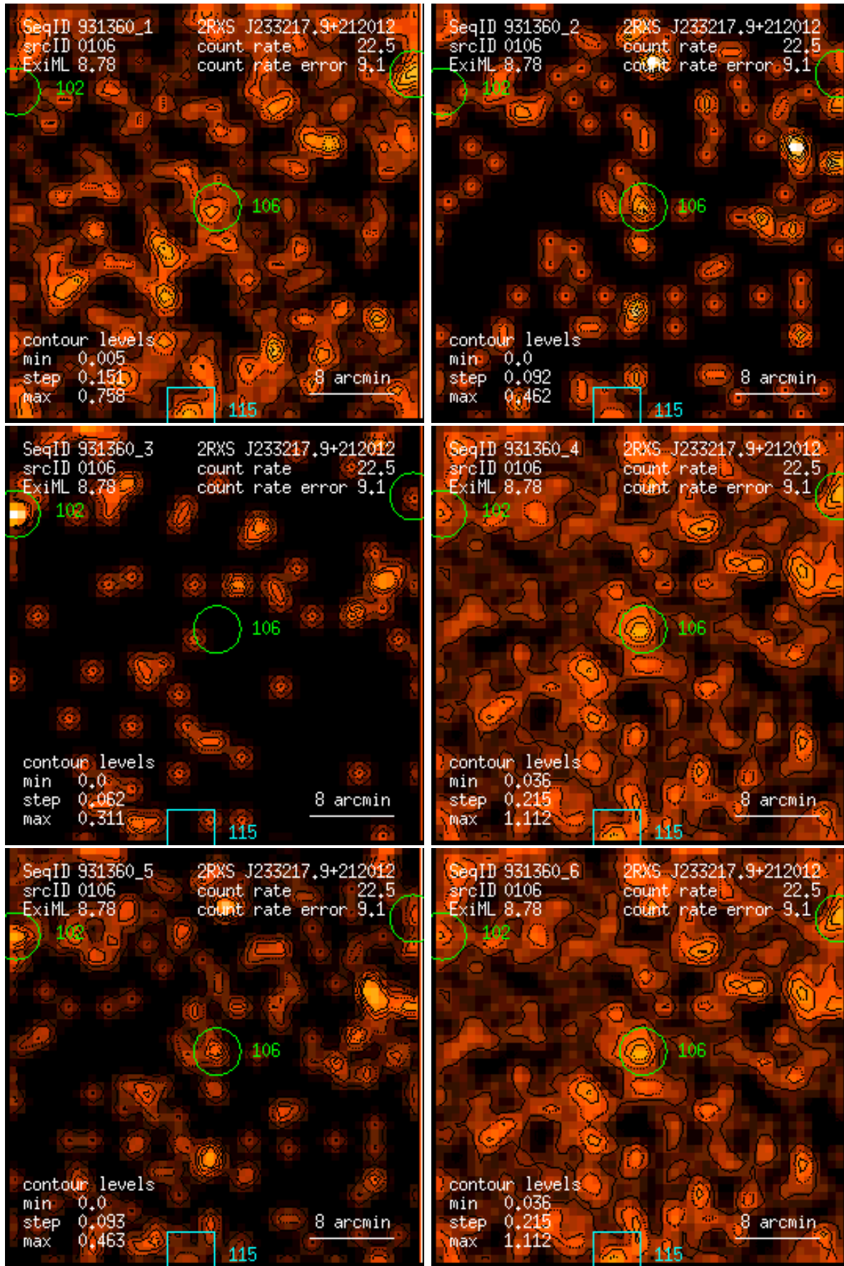
Figure 106: RASS 931360: detection 0106: band rate images, Gaussian filter: (1) PSPC channels 11 – 41, (2) 52 – 90, (3) 91 – 201, (4) 11 – 235, (5) 52 – 201, (6) 11 – 201. Broad band rates in counts/ks. Band rate contour levels in counts/ks/arcmin 2 .
