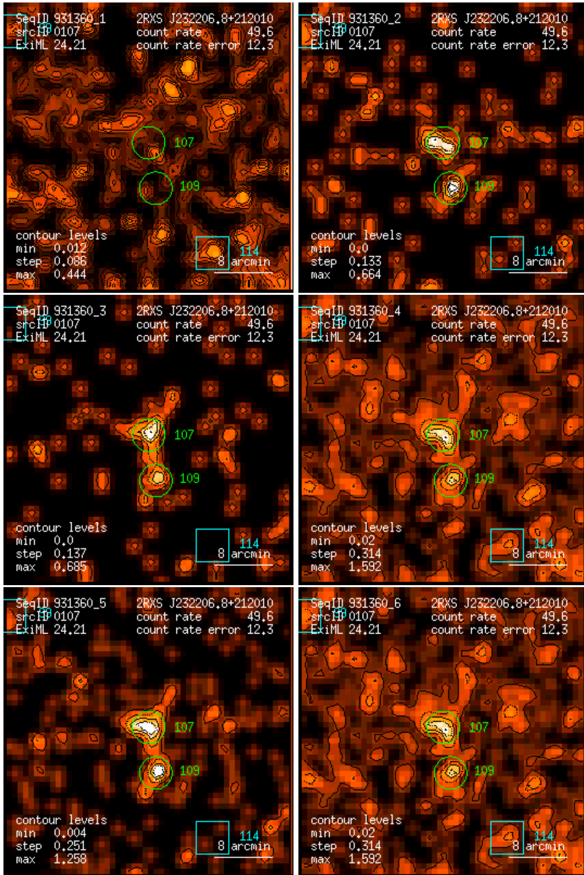
Figure 107: RASS 931360: detection 0107: band rate images, Gaussian filter: (1) PSPC channels 11 – 41, (2) 52 – 90, (3) 91 – 201, (4) 11 – 235, (5) 52 – 201, (6) 11 – 201. Broad band rates in counts/ks. Band rate contour levels in counts/ks/arcmin 2 .
