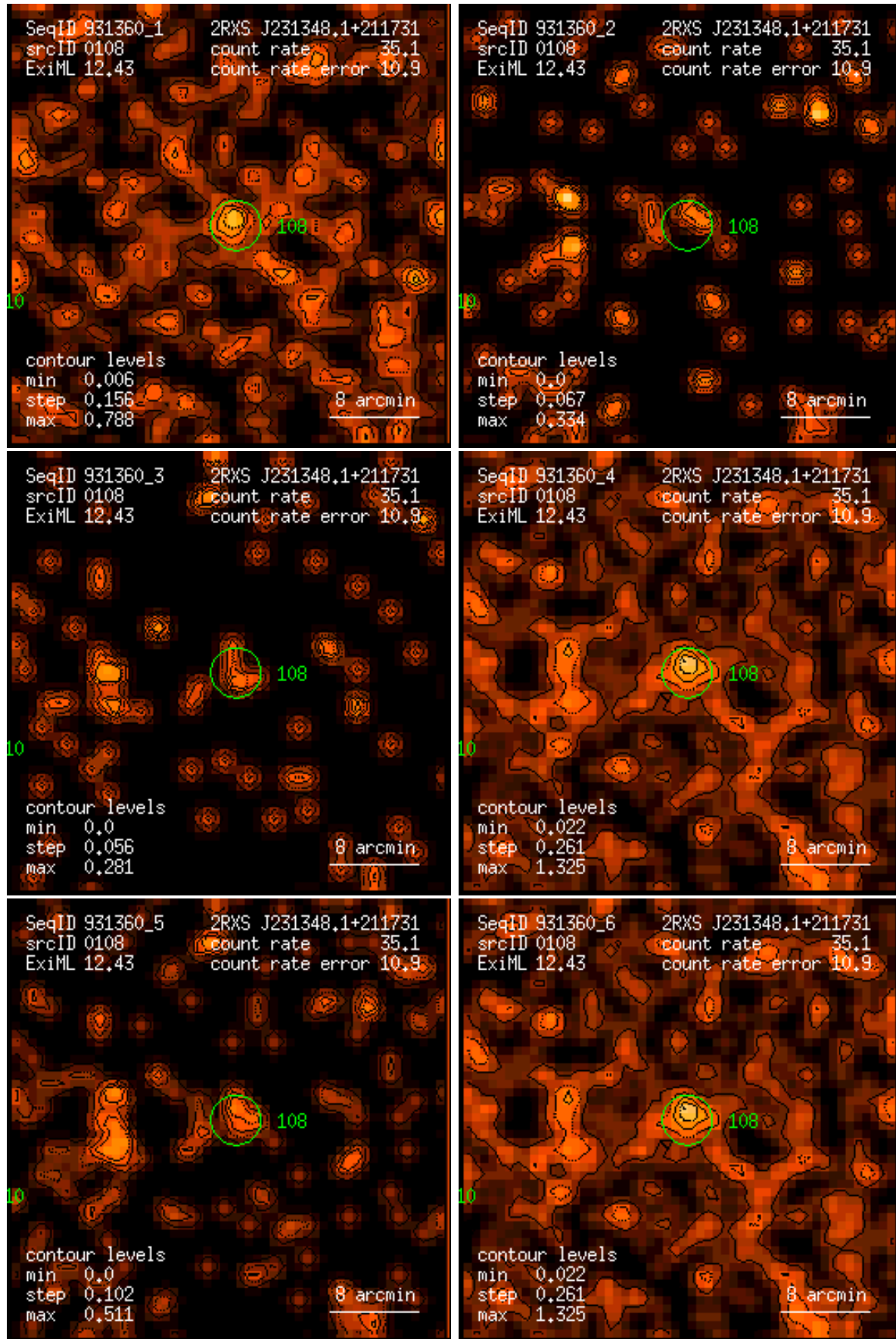
Figure 108: RASS 931360: detection 0108: band rate images, Gaussian filter: (1) PSPC channels 11 – 41, (2) 52 – 90, (3) 91 – 201, (4) 11 – 235, (5) 52 – 201, (6) 11 – 201. Broad band rates in counts/ks. Band rate contour levels in counts/ks/arcmin 2 .
