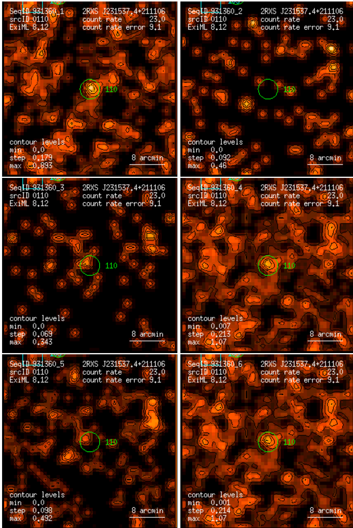
Figure 110: RASS 931360: detection 0110: band rate images, Gaussian filter: (1) PSPC channels 11 – 41, (2) 52 – 90, (3) 91 – 201, (4) 11 – 235, (5) 52 – 201, (6) 11 – 201. Broad band rates in counts/ks. Band rate contour levels in counts/ks/arcmin 2 .
