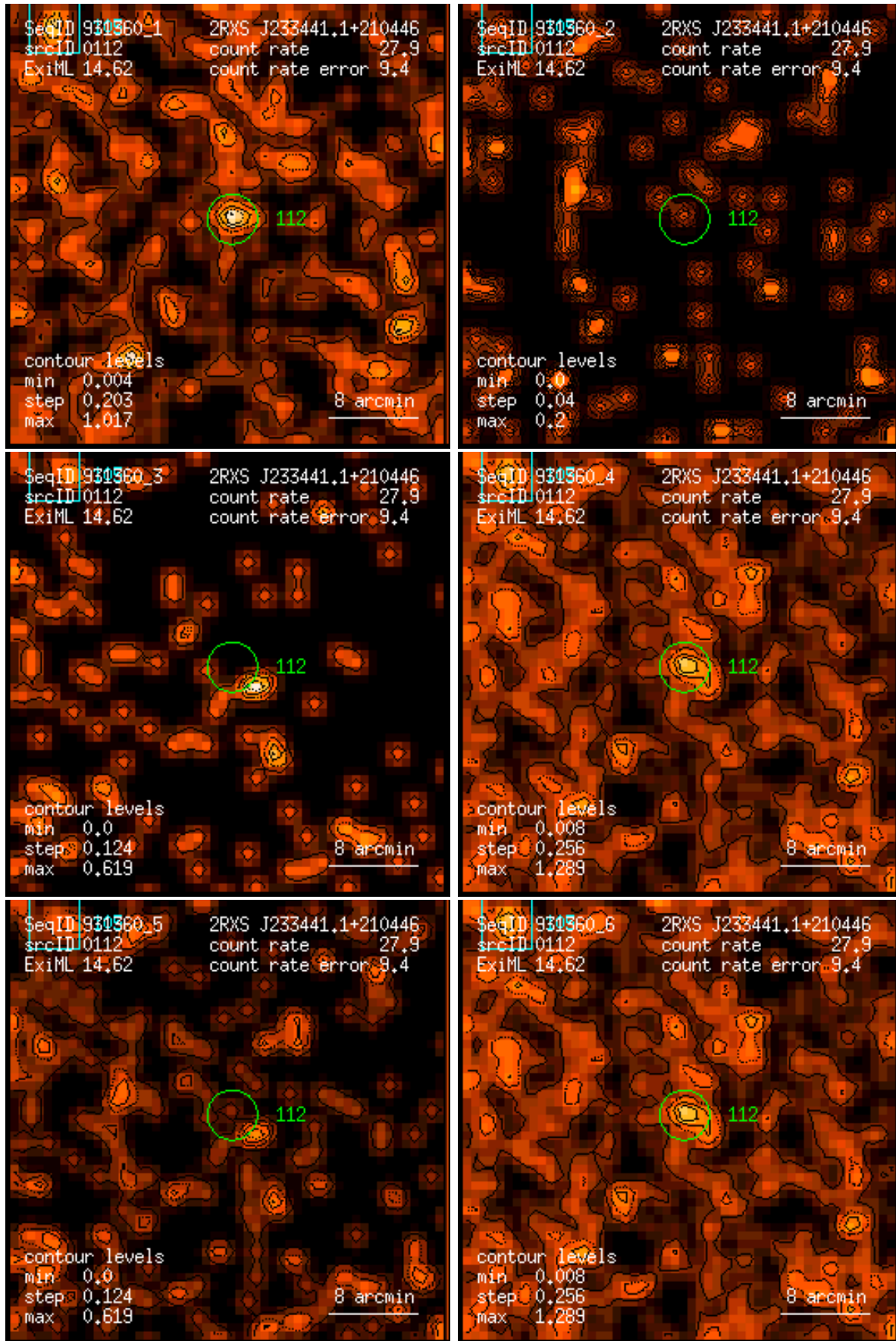
Figure 112: RASS 931360: detection 0112: band rate images, Gaussian filter: (1) PSPC channels 11 – 41, (2) 52 – 90, (3) 91 – 201, (4) 11 – 235, (5) 52 – 201, (6) 11 – 201. Broad band rates in counts/ks. Band rate contour levels in counts/ks/arcmin 2 .
