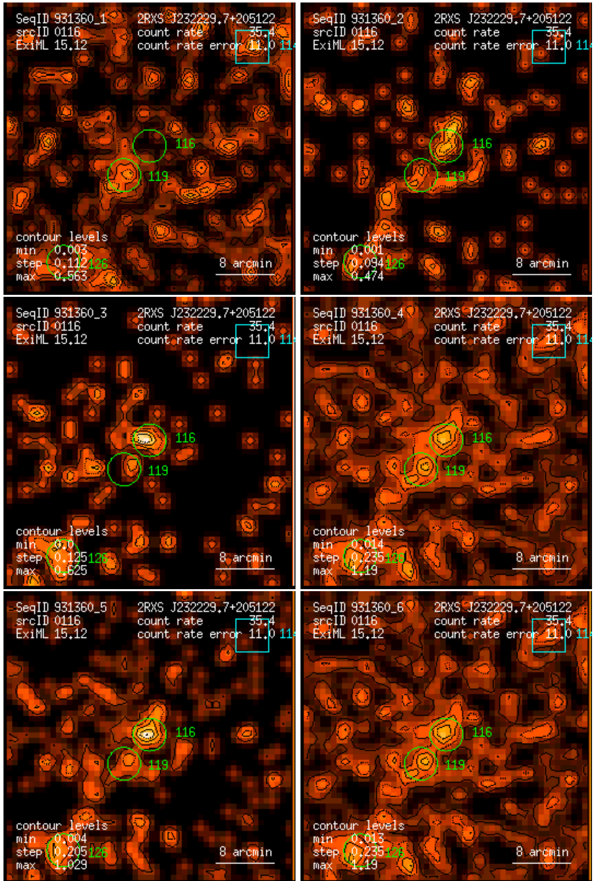
Figure 116: RASS 931360: detection 0116: band rate images, Gaussian filter: (1) PSPC channels 11 – 41, (2) 52 – 90, (3) 91 – 201, (4) 11 – 235, (5) 52 – 201, (6) 11 – 201. Broad band rates in counts/ks. Band rate contour levels in counts/ks/arcmin 2 .
