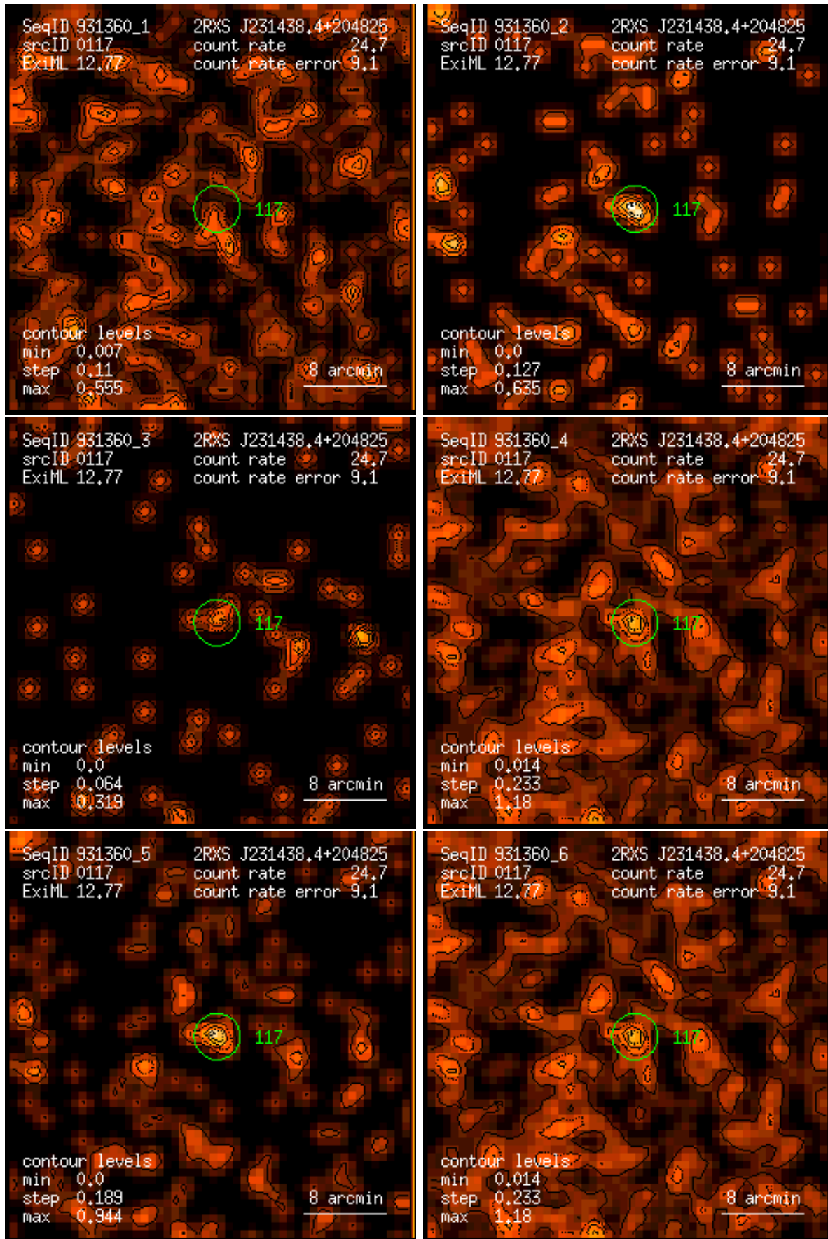
Figure 117: RASS 931360: detection 0117: band rate images, Gaussian filter: (1) PSPC channels 11 – 41, (2) 52 – 90, (3) 91 – 201, (4) 11 – 235, (5) 52 – 201, (6) 11 – 201. Broad band rates in counts/ks. Band rate contour levels in counts/ks/arcmin 2 .
