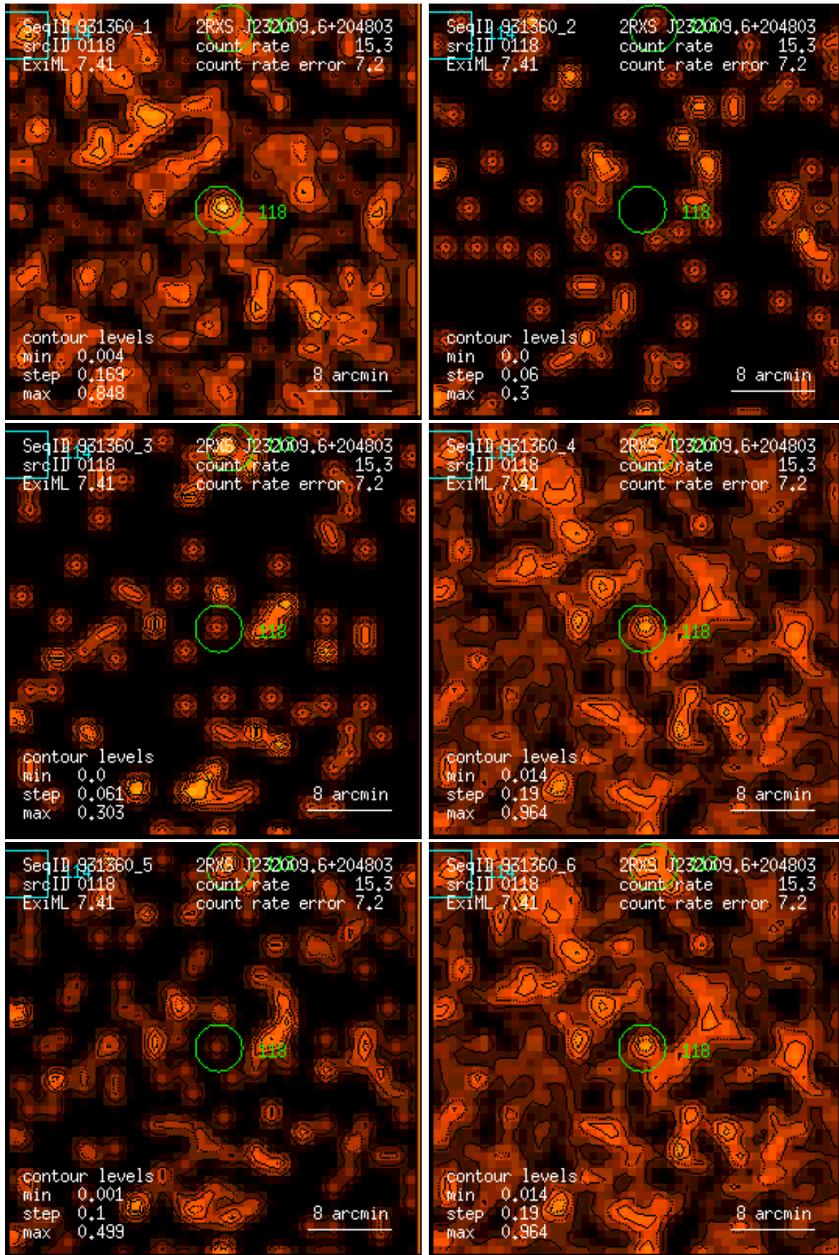
Figure 118: RASS 931360: detection 0118: band rate images, Gaussian filter: (1) PSPC channels 11 – 41, (2) 52 – 90, (3) 91 – 201, (4) 11 – 235, (5) 52 – 201, (6) 11 – 201. Broad band rates in counts/ks. Band rate contour levels in counts/ks/arcmin 2 .
