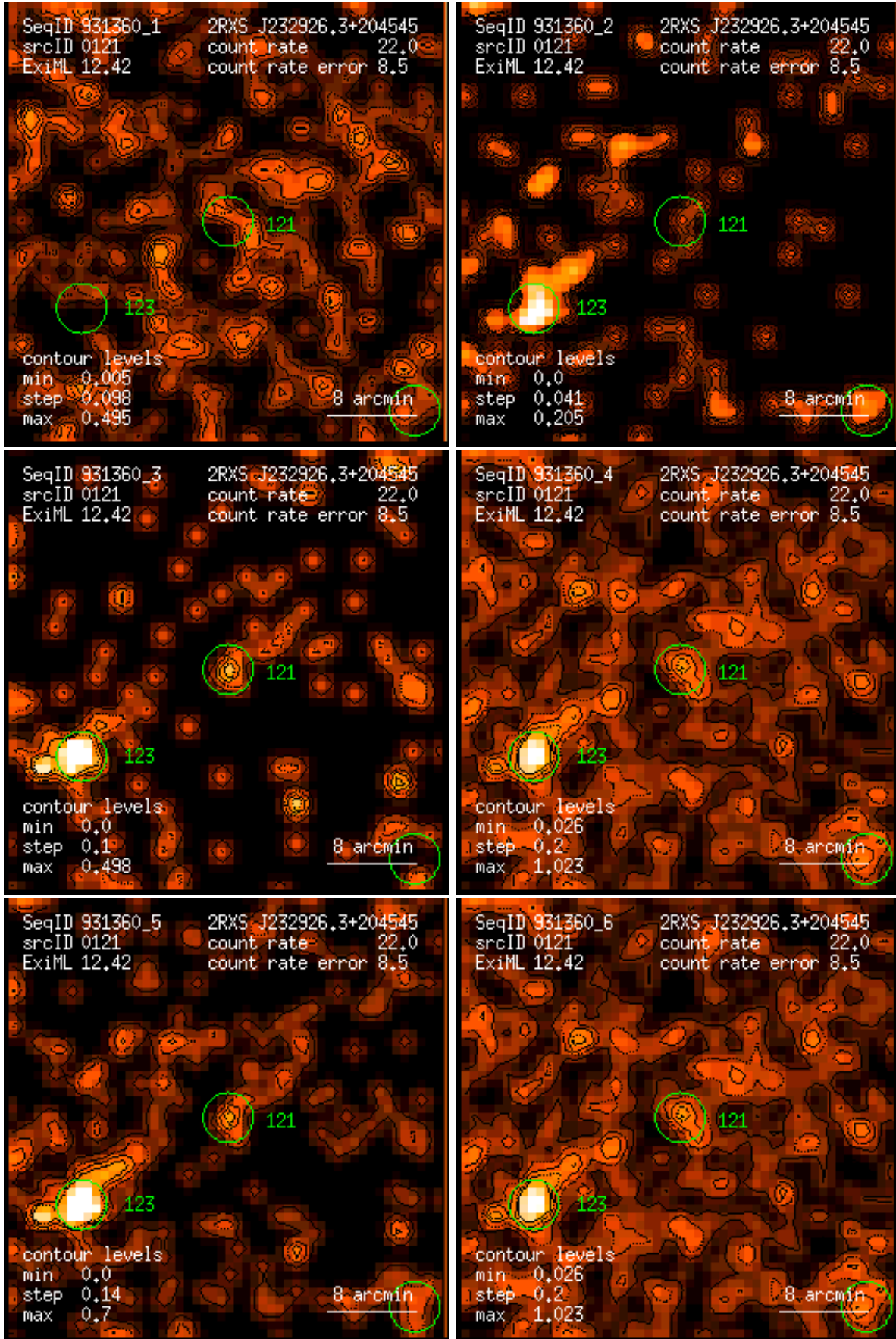
Figure 121: RASS 931360: detection 0121: band rate images, Gaussian filter: (1) PSPC channels 11 – 41, (2) 52 – 90, (3) 91 – 201, (4) 11 – 235, (5) 52 – 201, (6) 11 – 201. Broad band rates in counts/ks. Band rate contour levels in counts/ks/arcmin 2 .
