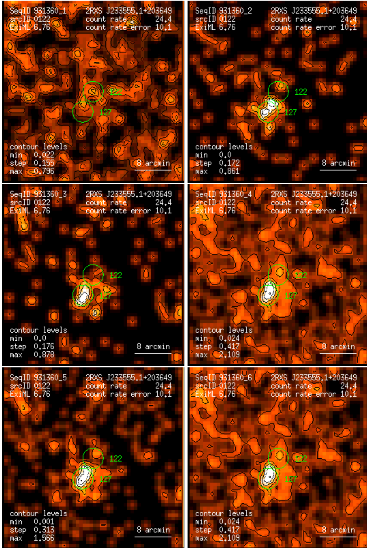
Figure 122: RASS 931360: detection 0122: band rate images, Gaussian filter: (1) PSPC channels 11 – 41, (2) 52 – 90, (3) 91 – 201, (4) 11 – 235, (5) 52 – 201, (6) 11 – 201. Broad band rates in counts/ks. Band rate contour levels in counts/ks/arcmin 2 .
