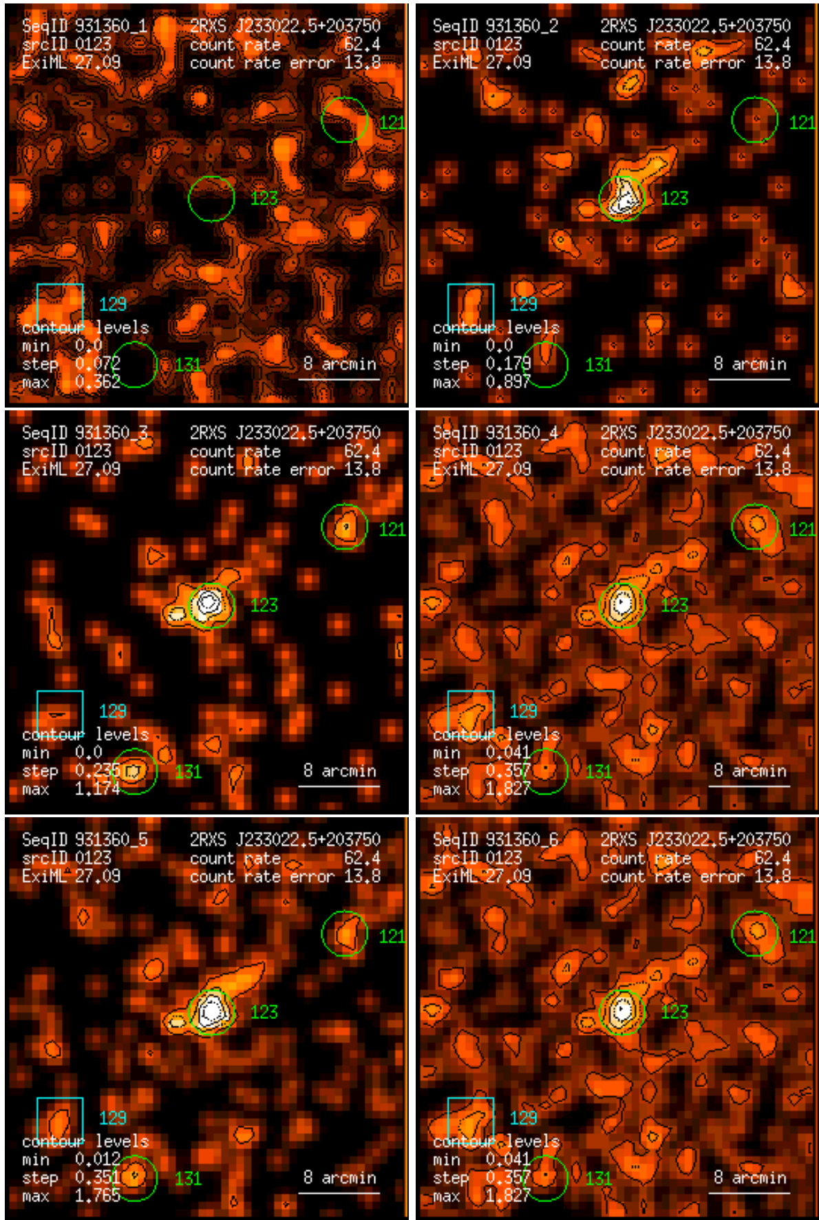
Figure 123: RASS 931360: detection 0123: band rate images, Gaussian filter: (1) PSPC channels 11 – 41, (2) 52 – 90, (3) 91 – 201, (4) 11 – 235, (5) 52 – 201, (6) 11 – 201. Broad band rates in counts/ks. Band rate contour levels in counts/ks/arcmin 2 .
