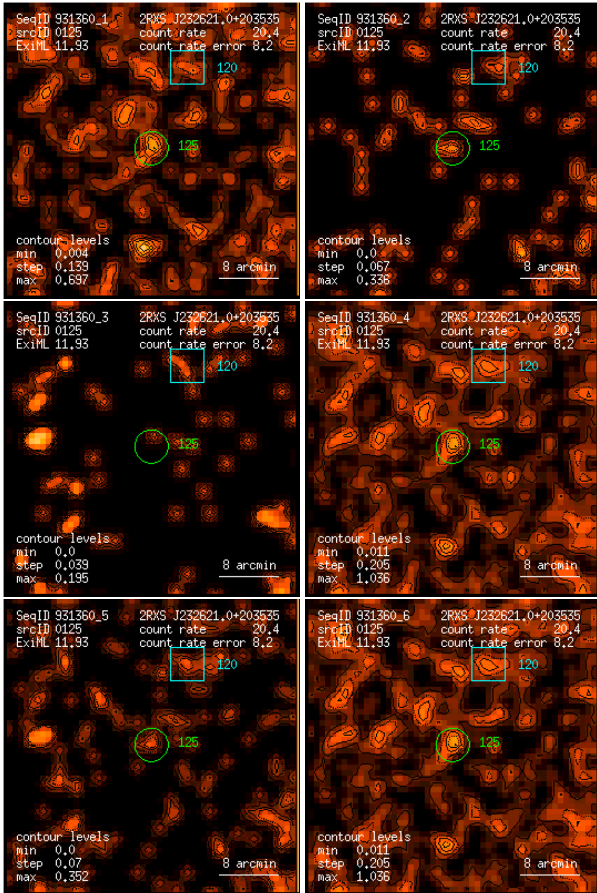
Figure 125: RASS 931360: detection 0125: band rate images, Gaussian filter: (1) PSPC channels 11 – 41, (2) 52 – 90, (3) 91 – 201, (4) 11 – 235, (5) 52 – 201, (6) 11 – 201. Broad band rates in counts/ks. Band rate contour levels in counts/ks/arcmin 2 .
