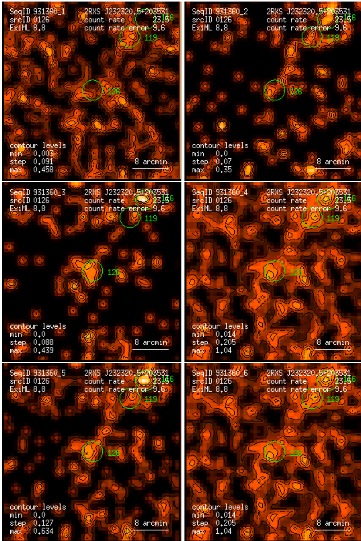
Figure 126: RASS 931360: detection 0126: band rate images, Gaussian filter: (1) PSPC channels 11 – 41, (2) 52 – 90, (3) 91 – 201, (4) 11 – 235, (5) 52 – 201, (6) 11 – 201. Broad band rates in counts/ks. Band rate contour levels in counts/ks/arcmin 2 .
