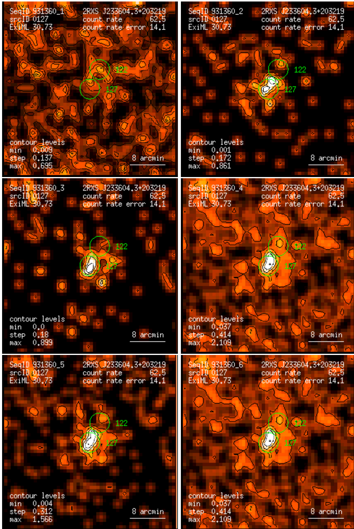
Figure 127: RASS 931360: detection 0127: band rate images, Gaussian filter: (1) PSPC channels 11 – 41, (2) 52 – 90, (3) 91 – 201, (4) 11 – 235, (5) 52 – 201, (6) 11 – 201. Broad band rates in counts/ks. Band rate contour levels in counts/ks/arcmin 2 .
