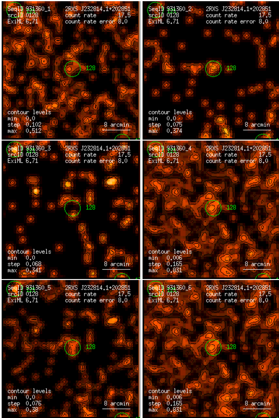
Figure 128: RASS 931360: detection 0128: band rate images, Gaussian filter: (1) PSPC channels 11 – 41, (2) 52 – 90, (3) 91 – 201, (4) 11 – 235, (5) 52 – 201, (6) 11 – 201. Broad band rates in counts/ks. Band rate contour levels in counts/ks/arcmin 2 .
