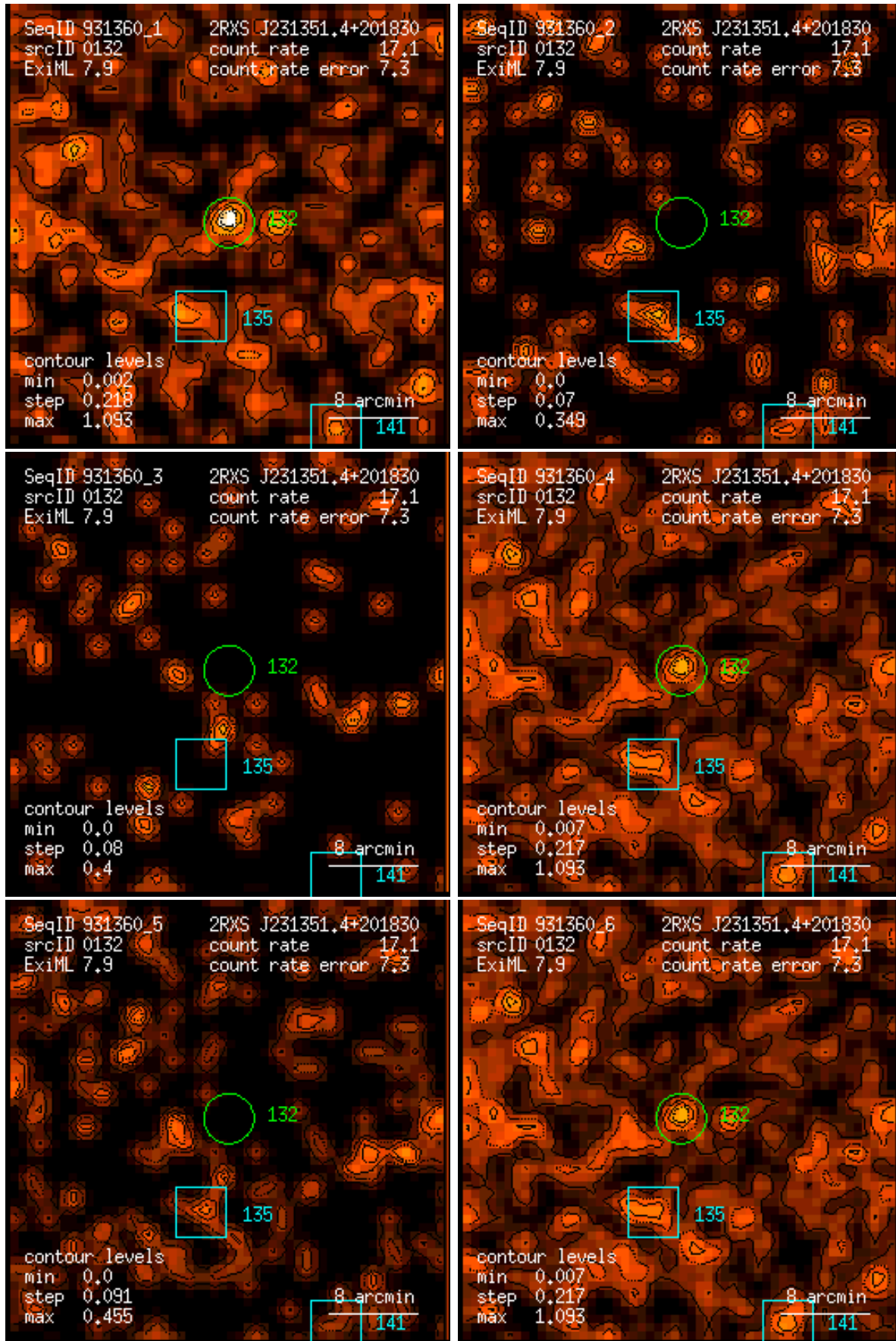
Figure 132: RASS 931360: detection 0132: band rate images, Gaussian filter: (1) PSPC channels 11 – 41, (2) 52 – 90, (3) 91 – 201, (4) 11 – 235, (5) 52 – 201, (6) 11 – 201. Broad band rates in counts/ks. Band rate contour levels in counts/ks/arcmin 2 .
