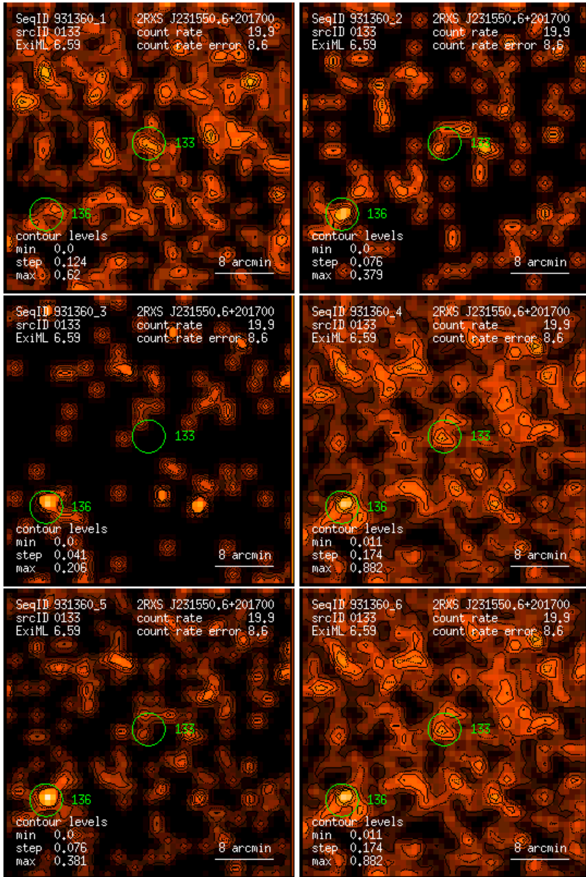
Figure 133: RASS 931360: detection 0133: band rate images, Gaussian filter: (1) PSPC channels 11 – 41, (2) 52 – 90, (3) 91 – 201, (4) 11 – 235, (5) 52 – 201, (6) 11 – 201. Broad band rates in counts/ks. Band rate contour levels in counts/ks/arcmin 2 .
