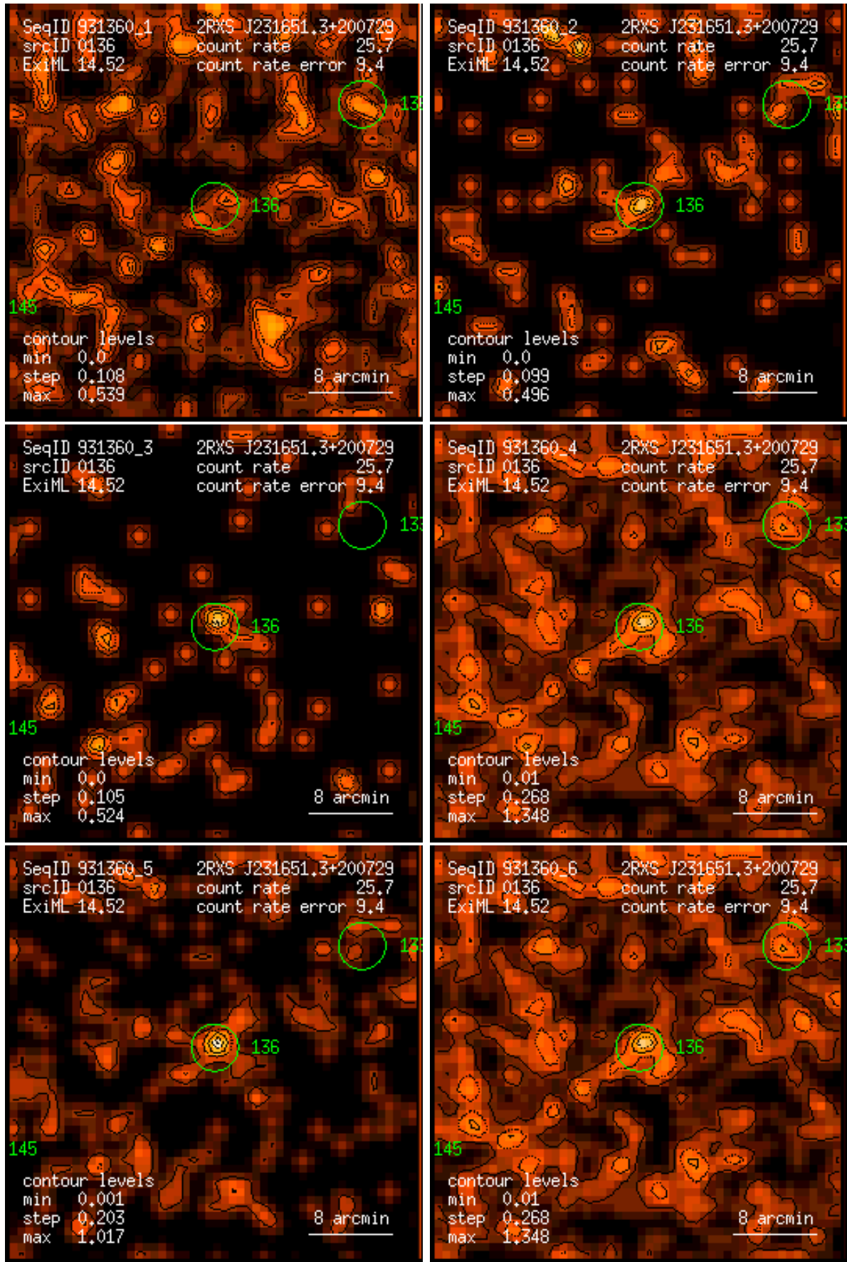
Figure 136: RASS 931360: detection 0136: band rate images, Gaussian filter: (1) PSPC channels 11 – 41, (2) 52 – 90, (3) 91 – 201, (4) 11 – 235, (5) 52 – 201, (6) 11 – 201. Broad band rates in counts/ks. Band rate contour levels in counts/ks/arcmin 2 .
