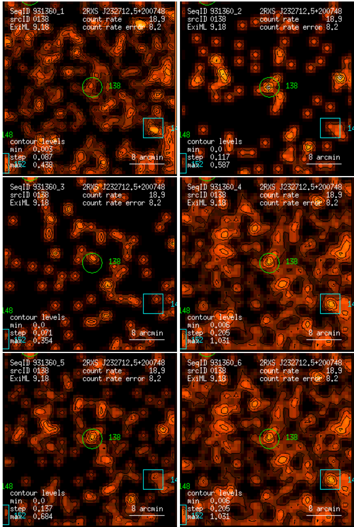
Figure 138: RASS 931360: detection 0138: band rate images, Gaussian filter: (1) PSPC channels 11 – 41, (2) 52 – 90, (3) 91 – 201, (4) 11 – 235, (5) 52 – 201, (6) 11 – 201. Broad band rates in counts/ks. Band rate contour levels in counts/ks/arcmin 2 .
