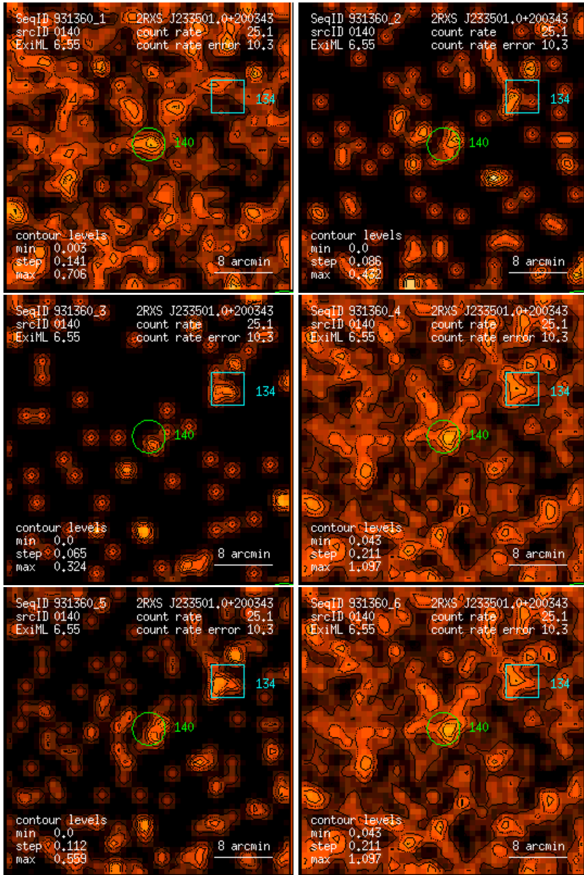
Figure 140: RASS 931360: detection 0140: band rate images, Gaussian filter: (1) PSPC channels 11 – 41, (2) 52 – 90, (3) 91 – 201, (4) 11 – 235, (5) 52 – 201, (6) 11 – 201. Broad band rates in counts/ks. Band rate contour levels in counts/ks/arcmin 2 .
