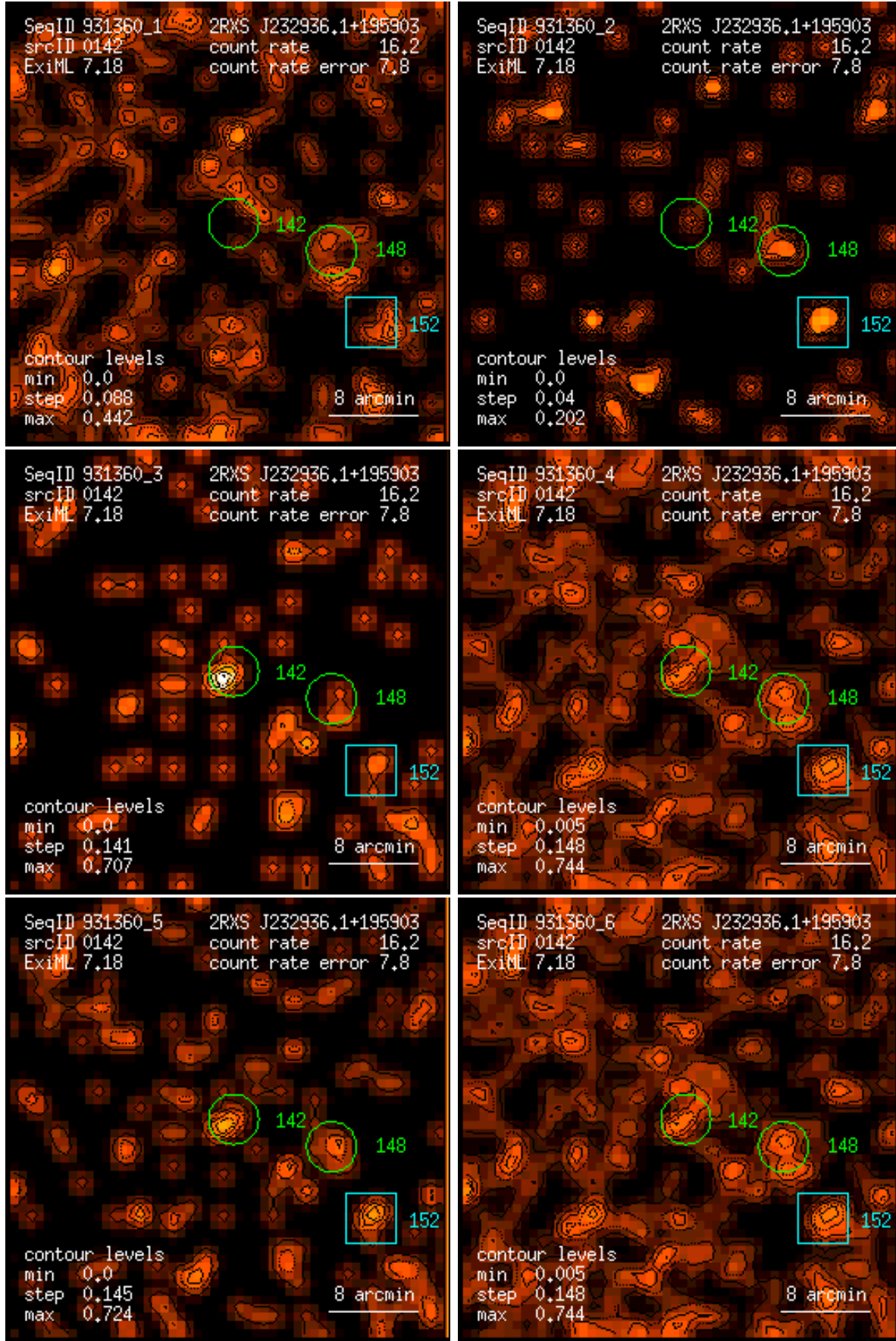
Figure 142: RASS 931360: detection 0142: band rate images, Gaussian filter: (1) PSPC channels 11 – 41, (2) 52 – 90, (3) 91 – 201, (4) 11 – 235, (5) 52 – 201, (6) 11 – 201. Broad band rates in counts/ks. Band rate contour levels in counts/ks/arcmin 2 .
