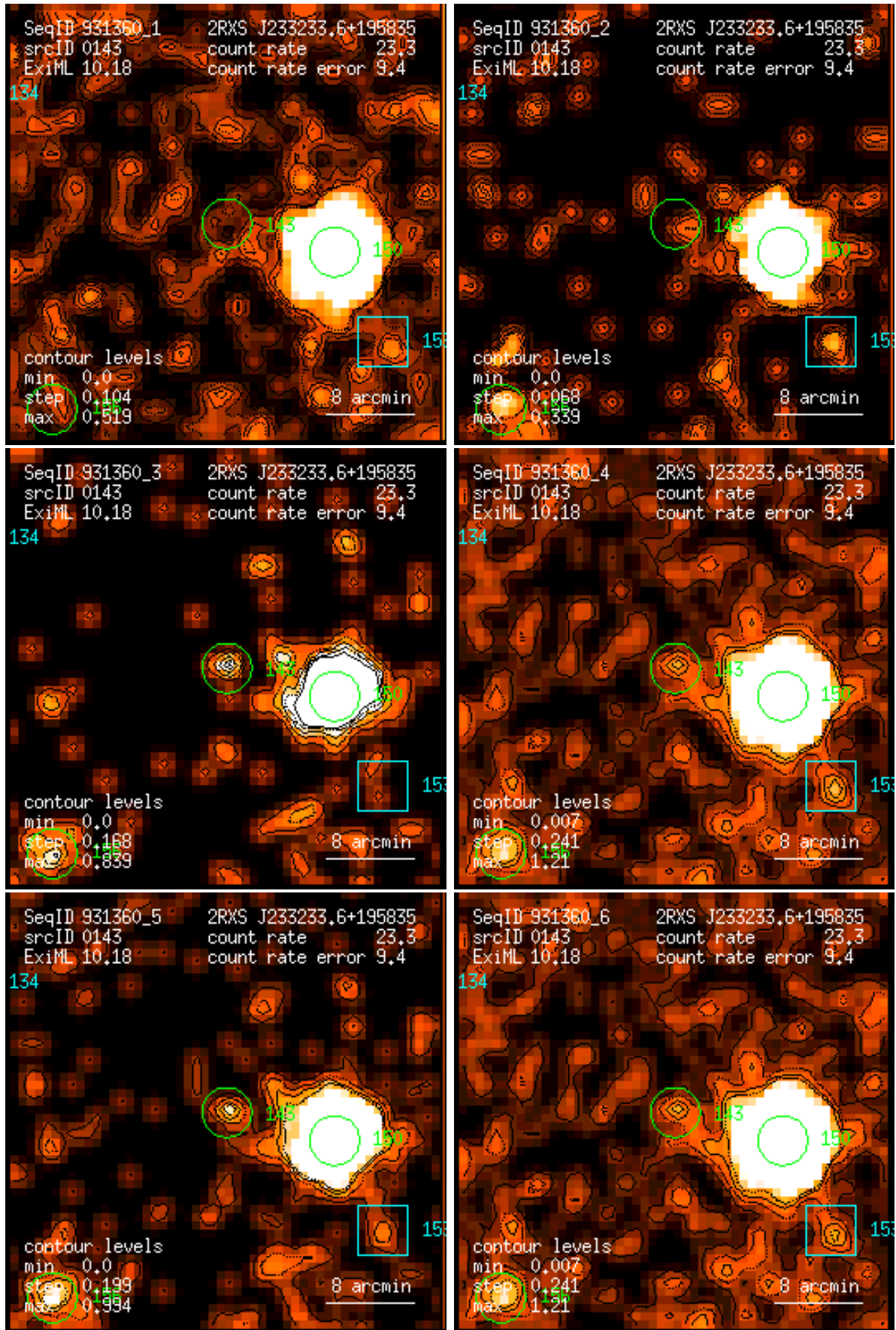
Figure 143: RASS 931360: detection 0143: band rate images, Gaussian filter: (1) PSPC channels 11 – 41, (2) 52 – 90, (3) 91 – 201, (4) 11 – 235, (5) 52 – 201, (6) 11 – 201. Broad band rates in counts/ks. Band rate contour levels in counts/ks/arcmin 2 .
