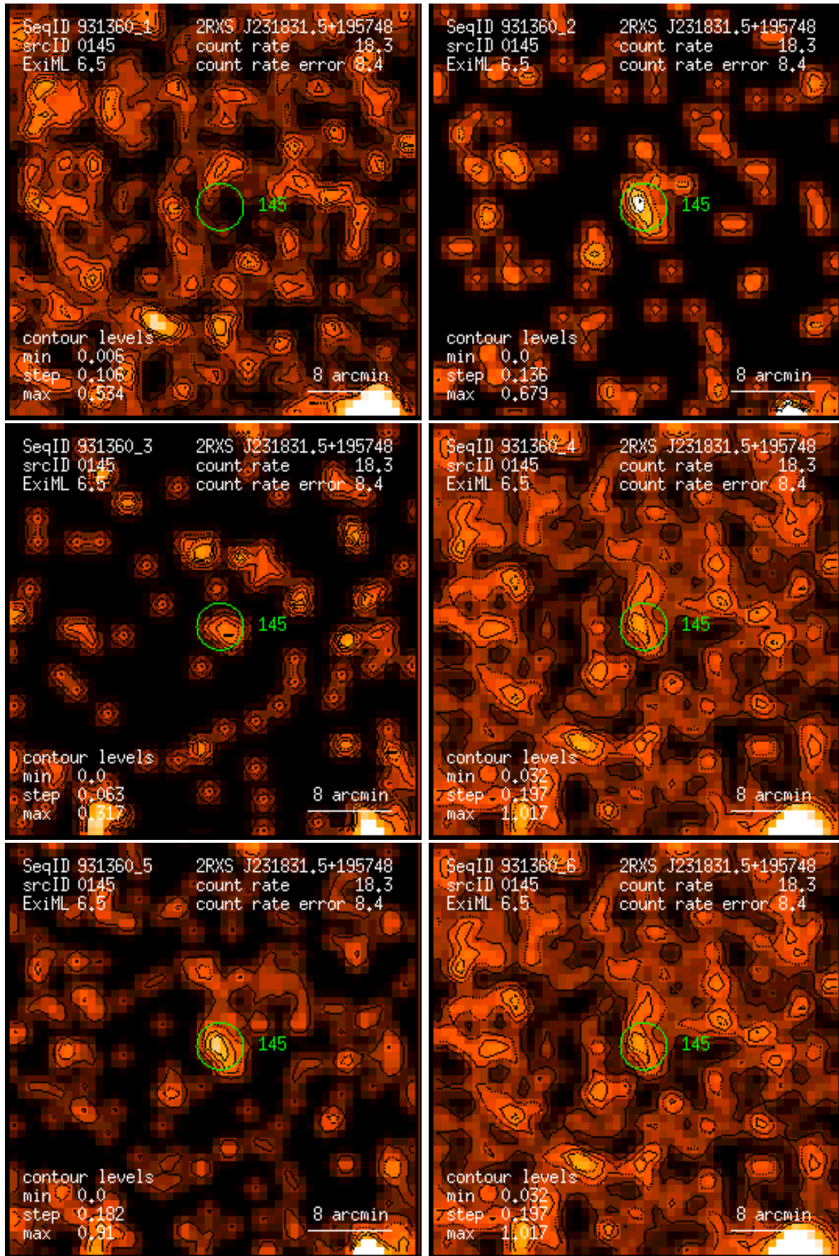
Figure 145: RASS 931360: detection 0145: band rate images, Gaussian filter: (1) PSPC channels 11 – 41, (2) 52 – 90, (3) 91 – 201, (4) 11 – 235, (5) 52 – 201, (6) 11 – 201. Broad band rates in counts/ks. Band rate contour levels in counts/ks/arcmin 2 .
