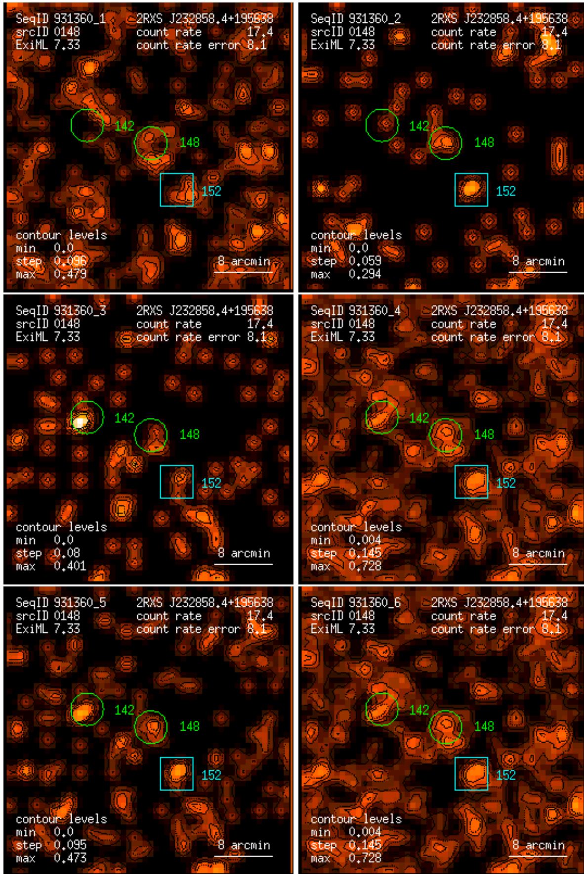
Figure 148: RASS 931360: detection 0148: band rate images, Gaussian filter: (1) PSPC channels 11 – 41, (2) 52 – 90, (3) 91 – 201, (4) 11 – 235, (5) 52 – 201, (6) 11 – 201. Broad band rates in counts/ks. Band rate contour levels in counts/ks/arcmin 2 .
