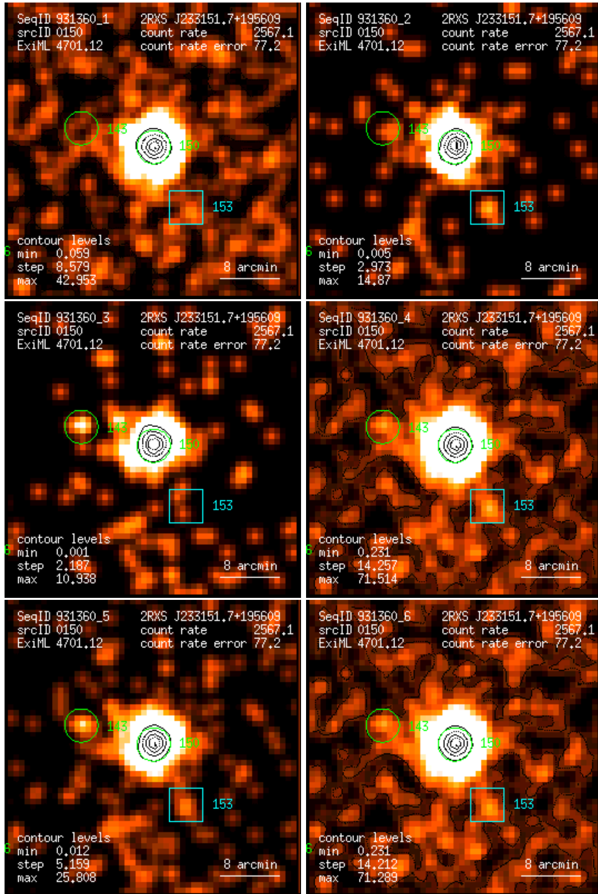
Figure 150: RASS 931360: detection 0150: band rate images, Gaussian filter: (1) PSPC channels 11 – 41, (2) 52 – 90, (3) 91 – 201, (4) 11 – 235, (5) 52 – 201, (6) 11 – 201. Broad band rates in counts/ks. Band rate contour levels in counts/ks/arcmin 2 .
