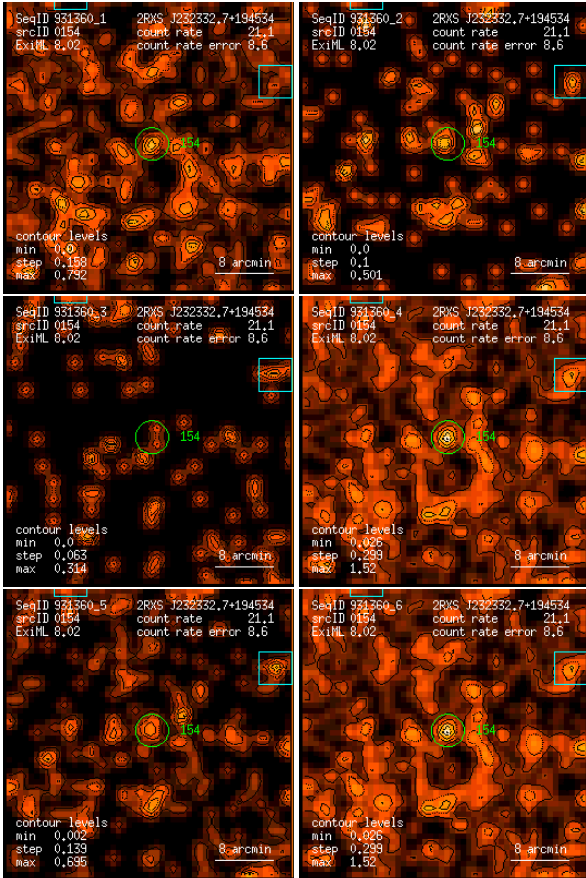
Figure 154: RASS 931360: detection 0154: band rate images, Gaussian filter: (1) PSPC channels 11 – 41, (2) 52 – 90, (3) 91 – 201, (4) 11 – 235, (5) 52 – 201, (6) 11 – 201. Broad band rates in counts/ks. Band rate contour levels in counts/ks/arcmin 2 .
