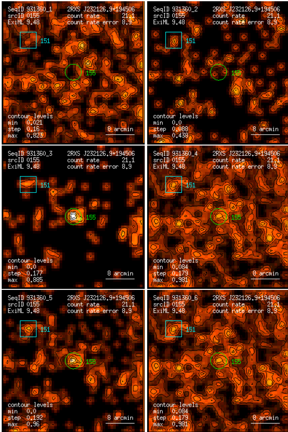
Figure 155: RASS 931360: detection 0155: band rate images, Gaussian filter: (1) PSPC channels 11 – 41, (2) 52 – 90, (3) 91 – 201, (4) 11 – 235, (5) 52 – 201, (6) 11 – 201. Broad band rates in counts/ks. Band rate contour levels in counts/ks/arcmin 2 .
