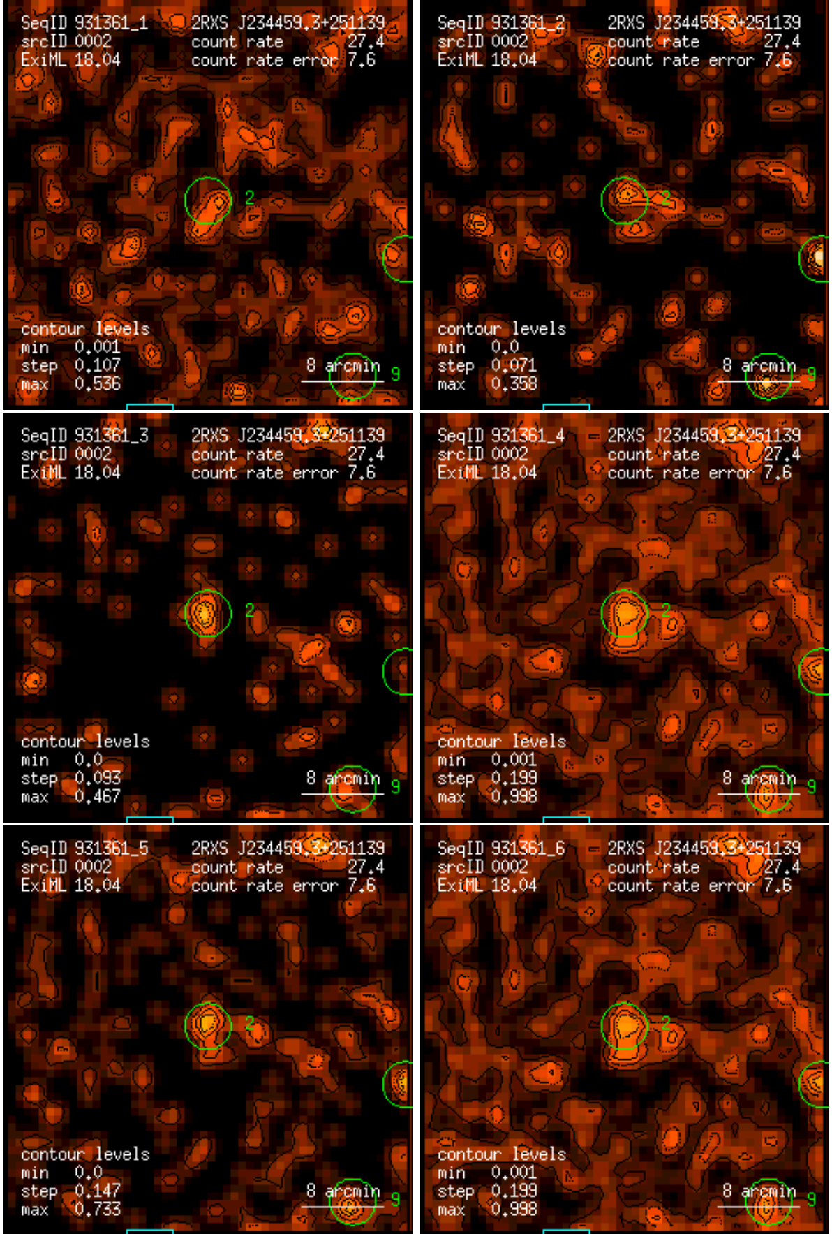
Figure 2: RASS 931361: detection 0002: band rate images, Gaussian filter: (1) PSPC channels 11 – 41, (2) 52 – 90, (3) 91 – 201, (4) 11 – 235, (5) 52 – 201, (6) 11 – 201. Broad band rates in counts/ks. Band rate contour levels in counts/ks/arcmin 2 .
