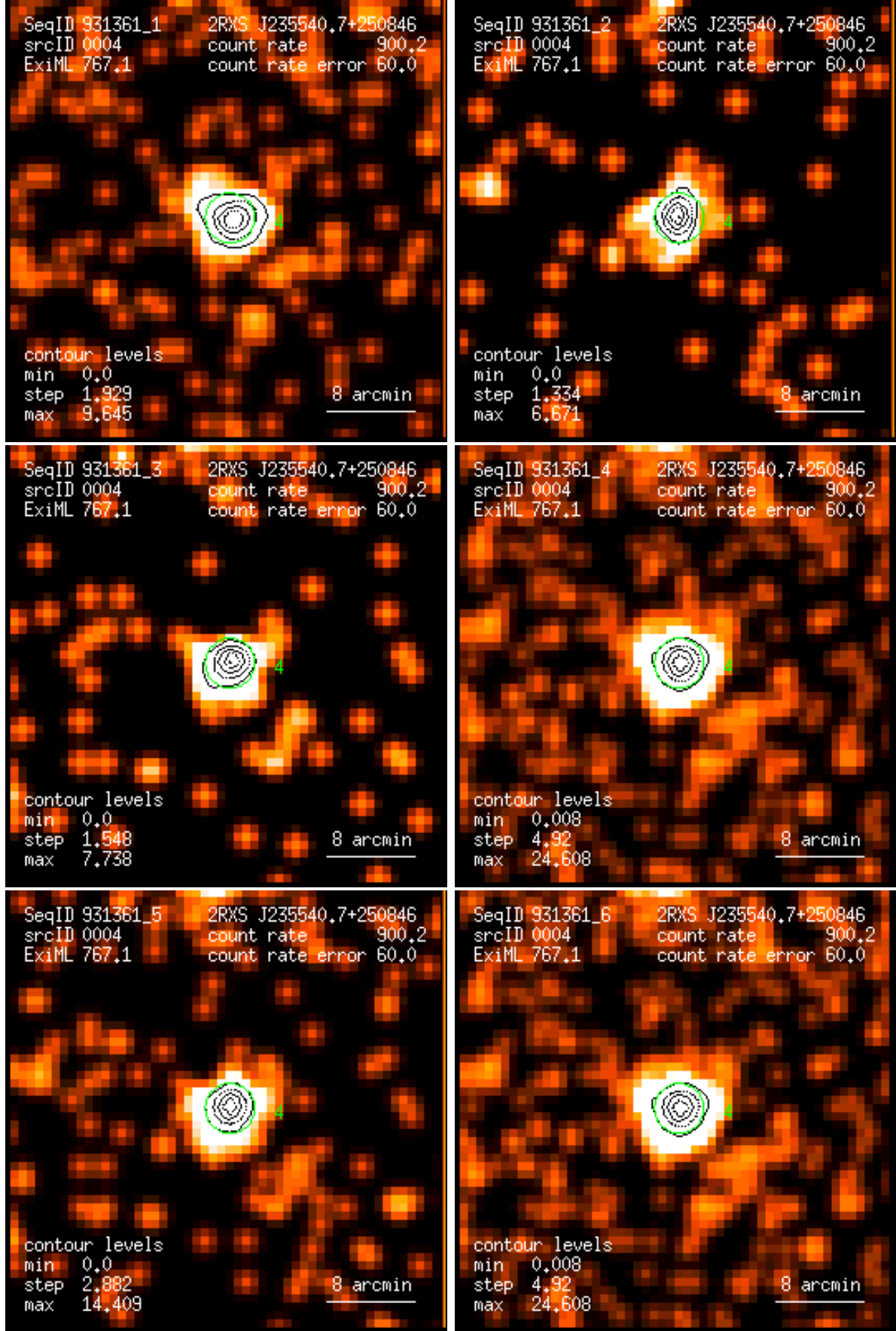
Figure 4: RASS 931361: detection 0004: band rate images, Gaussian filter: (1) PSPC channels 11 – 41, (2) 52 – 90, (3) 91 – 201, (4) 11 – 235, (5) 52 – 201, (6) 11 – 201. Broad band rates in counts/ks. Band rate contour levels in counts/ks/arcmin 2 .
