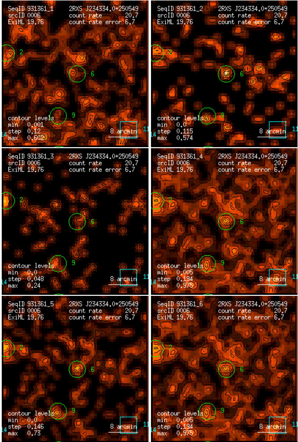
Figure 6: RASS 931361: detection 0006: band rate images, Gaussian filter: (1) PSPC channels 11 – 41, (2) 52 – 90, (3) 91 – 201, (4) 11 – 235, (5) 52 – 201, (6) 11 – 201. Broad band rates in counts/ks. Band rate contour levels in counts/ks/arcmin 2 .
